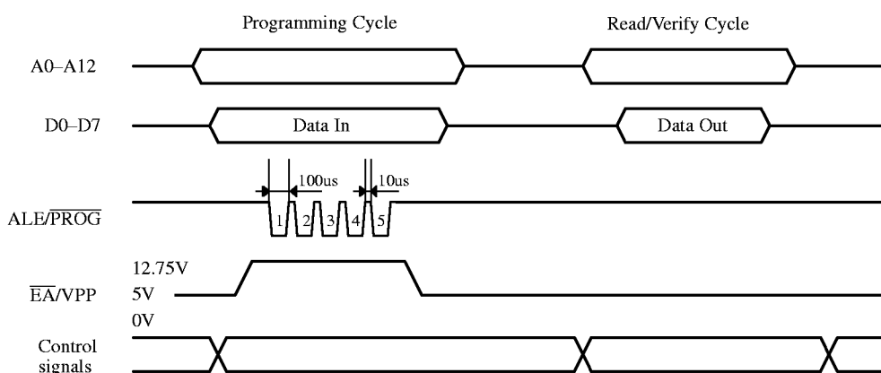
Figure 9 Programming and verification signal's waveform
