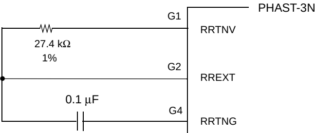
Figure 32. Clock Recovery External Component Connections
