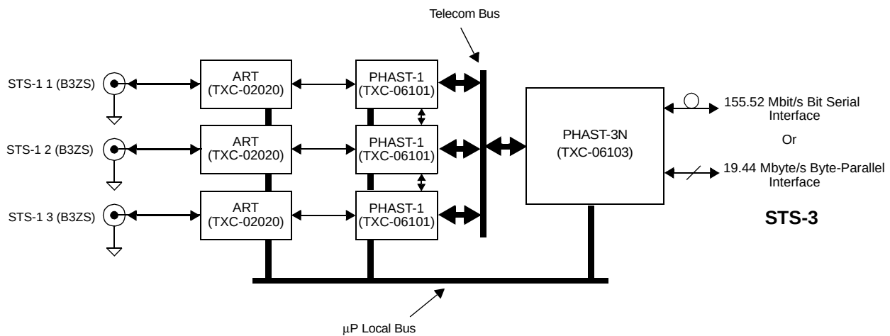
Figure 44. Mux of three STS 1 to/from one STS-3
