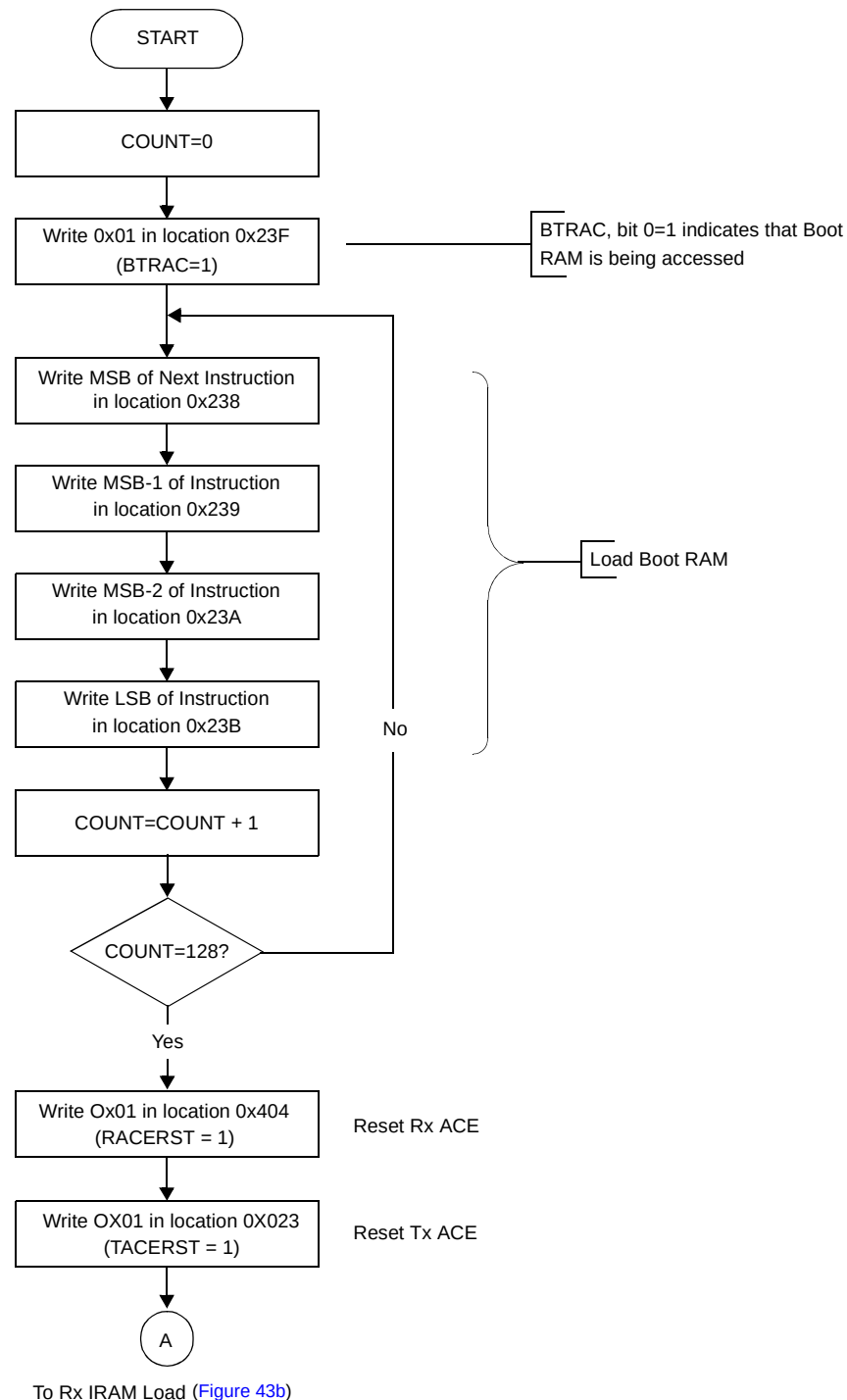
Figure 43a. Firmware Download Procedure Phase 1: Boot RAM Load
