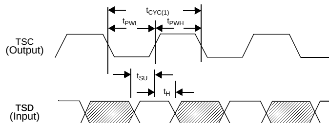
Figure 18. Transmit Section Data Communication Interface Timing (D1-D3 Bytes)
