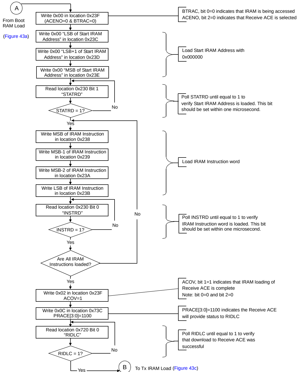
Figure 43b. Firmware Download Procedure Phase 2: Rx IRAM Load
