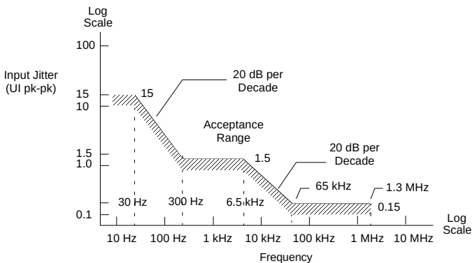
Figure 31. Clock Recovery Jitter Tolerance (per GR-253-CORE, Issue 3, September 2000)
