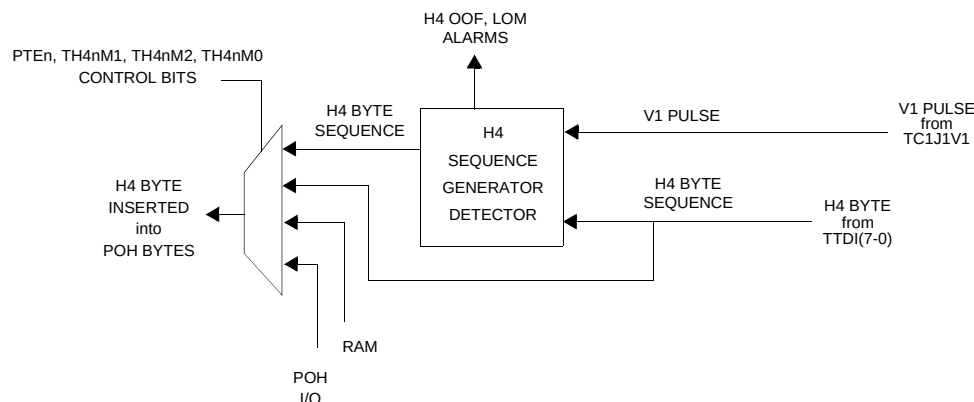
Figure 39. H4 Byte Functions in Normal Timing Mode
