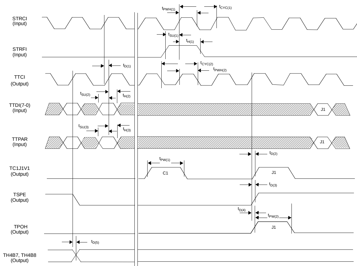
Figure 16. Transmit Terminal Interface Source Timing
