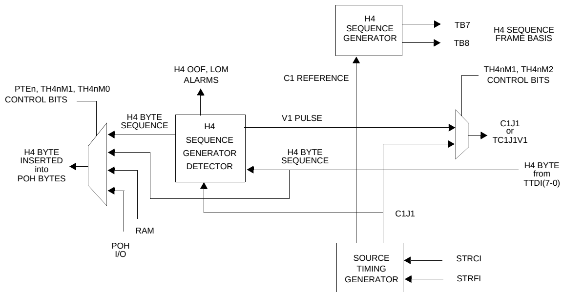
Figure 38. H4 Byte Functions in Source Timing Mode
