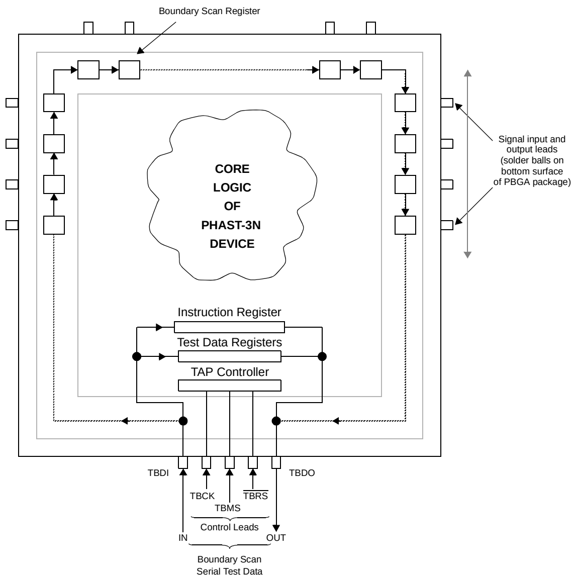
Boundary Scan Register
