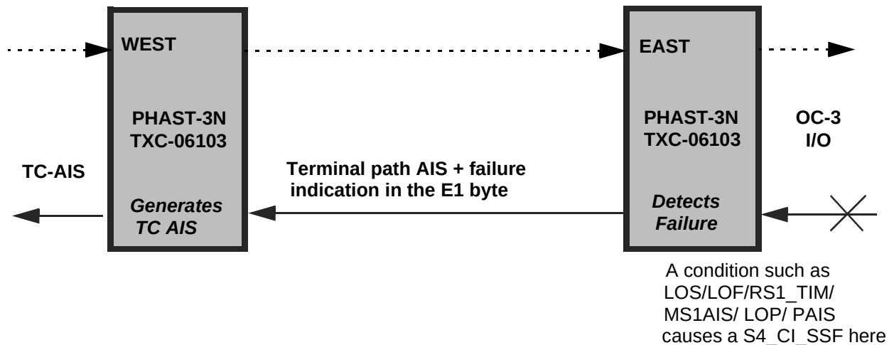
Figure 37. Transmission of TX-AIS During Failure
