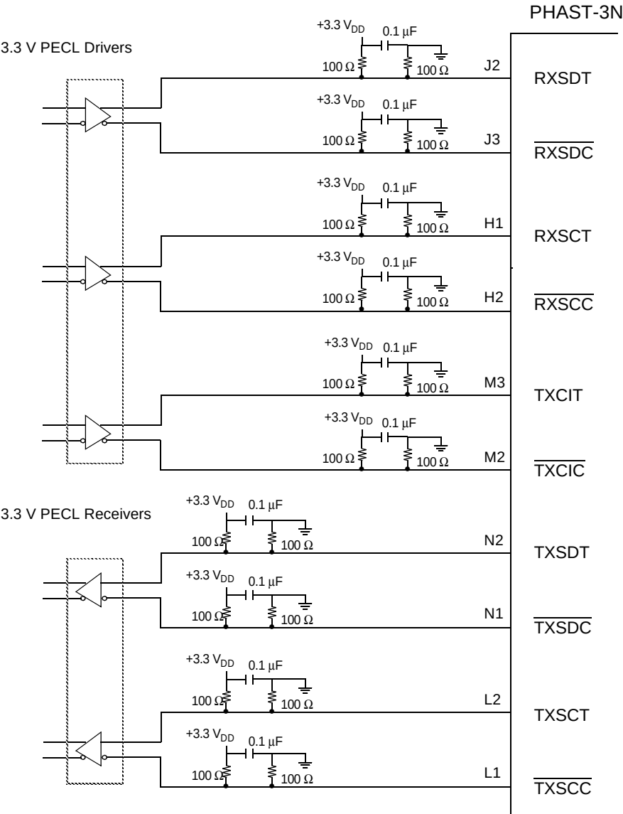
Figure 29. Termination of Pseudo-ECL Leads
