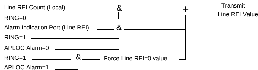
Figure 40. Transmit Line REI Count in M1 Byte Logic Diagram
