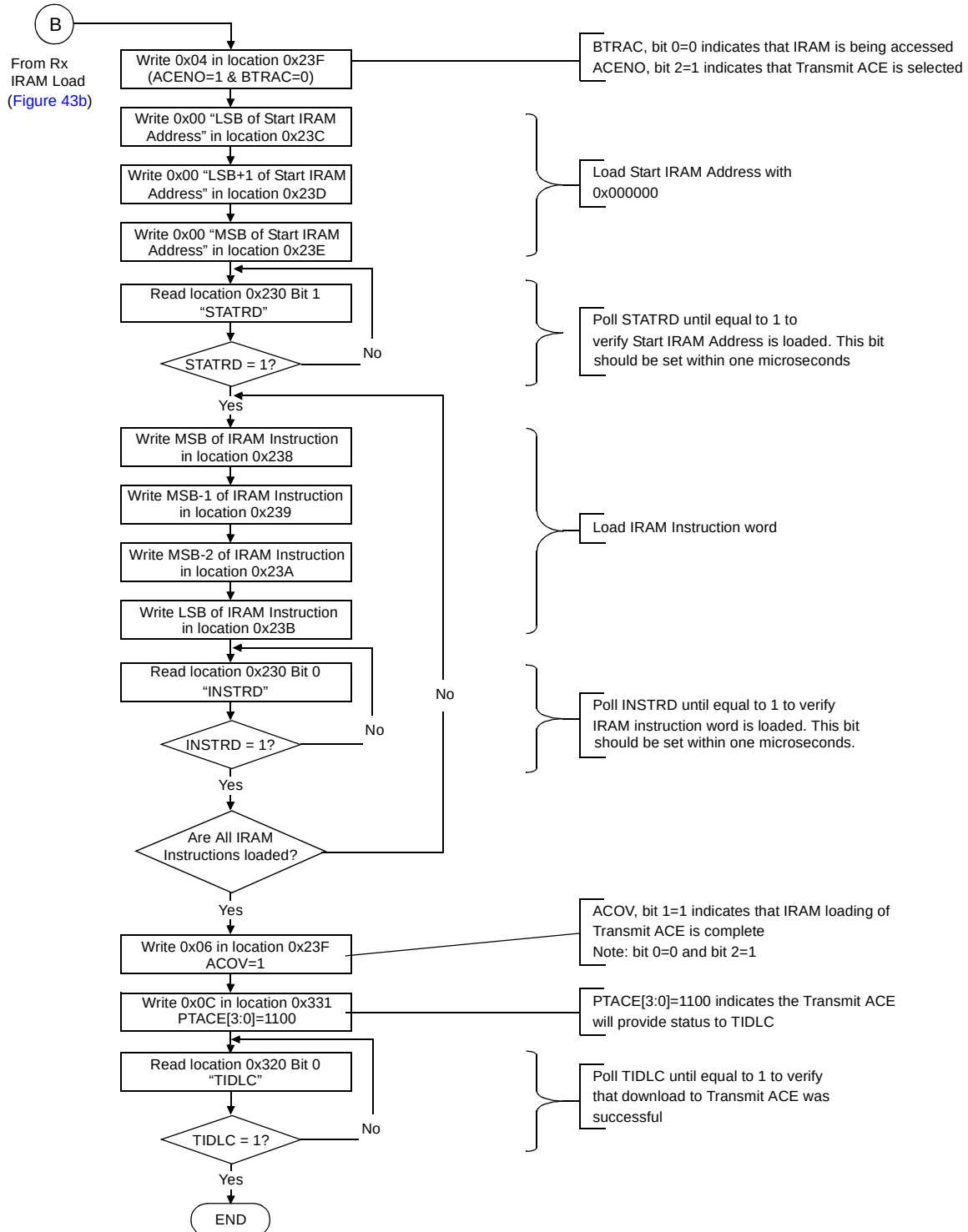
Figure 43c. Firmware Download Procedure Phase 3: Tx IRAM Load
