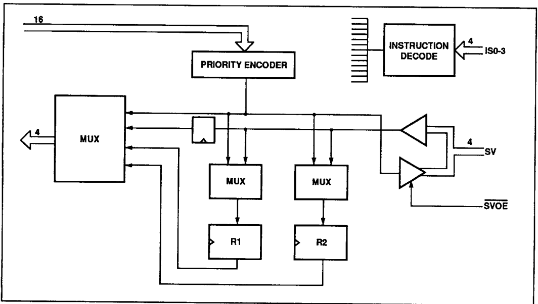
Fig.3 Shift control block
