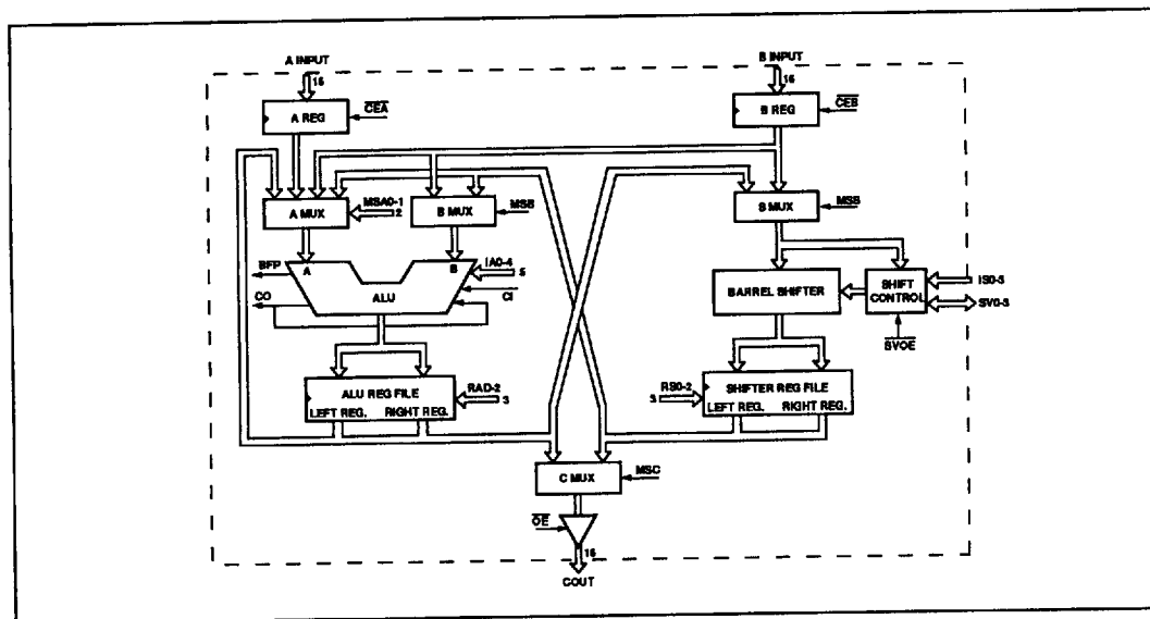
Fig.2 PDSP1601 block diagram
