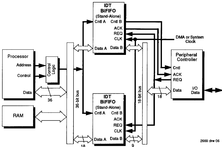
Figure 2. 36- to 18-Bit Peripheral Interface Configuration
