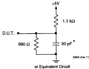
Figure 8. Output Load
