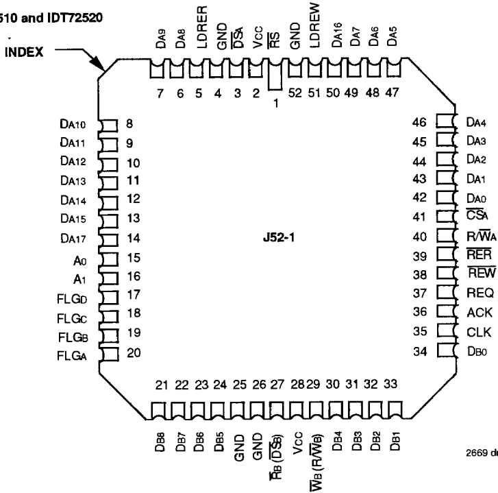
PLCC TOP VIEW
