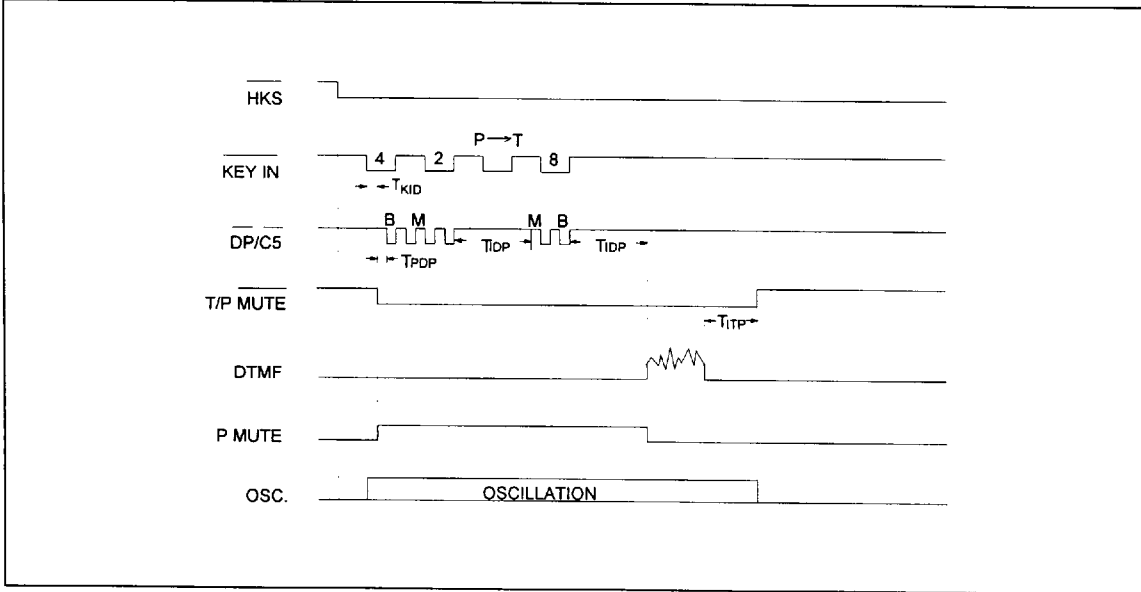
Figure 4. P->T Operation Timing Diagram in Normal Dialing
