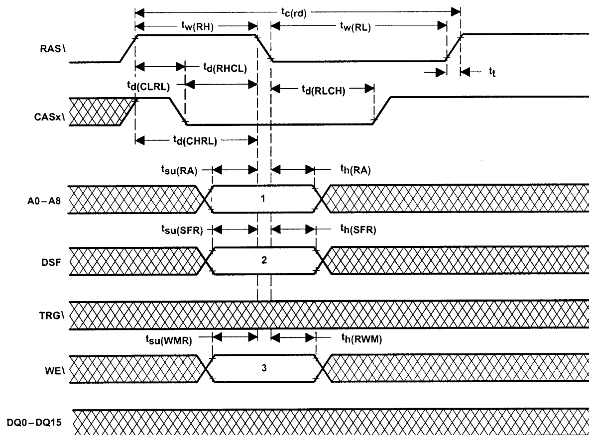
FIGURE 41: CBR-REFRESH-CYCLE TIMING
