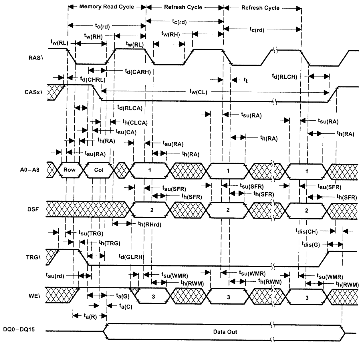
FIGURE 42: HIDDEN-REFRESH-CYCLE TIMING
