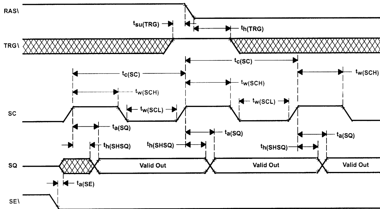
FIGURE 46: SERIAL-READ-CYCLE TIMING ( SE\downarrow = V_{IL} )
