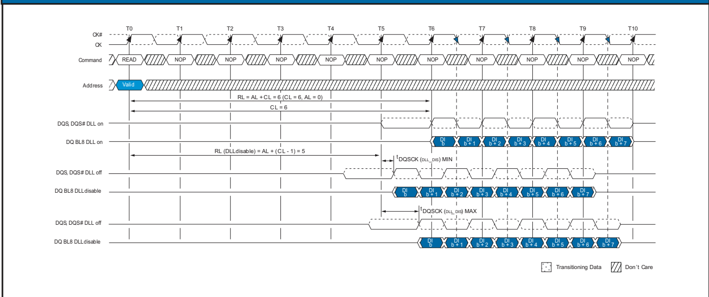
FIGURE 36 - DLL DISABLE t DQSK TIMING
