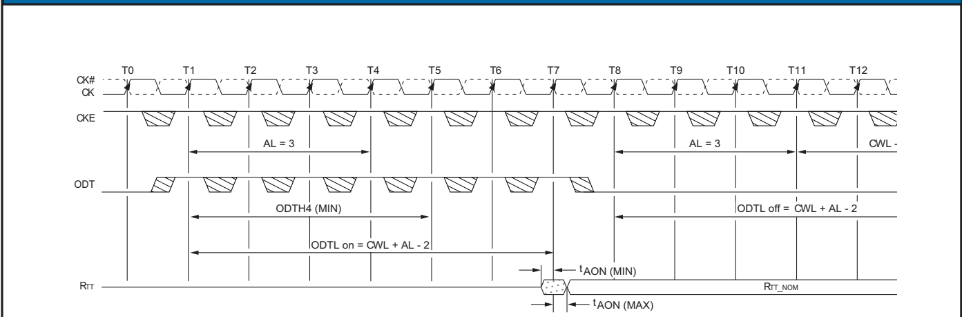
FIGURE 106 - SYNCHRONOUS ODT
