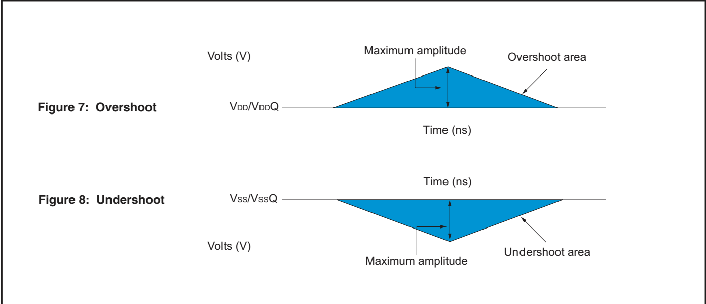
FIGURE 7 & 8: OVERSHOOT/UNDERSHOOT SPECIFICATIONS
