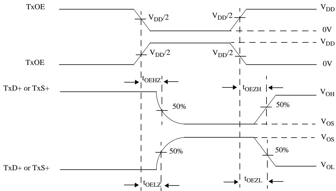
Figure 4. Output Enable to Data Out Timing
