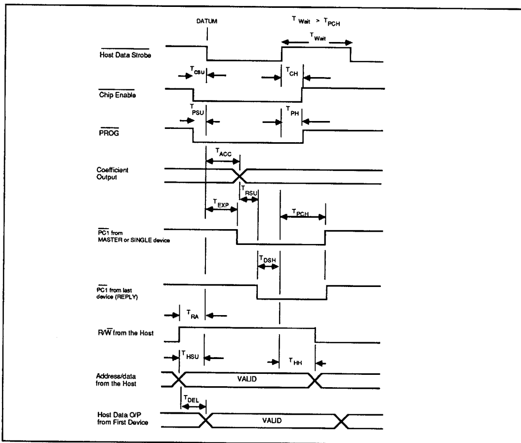
FIG. 8. Host Timing
