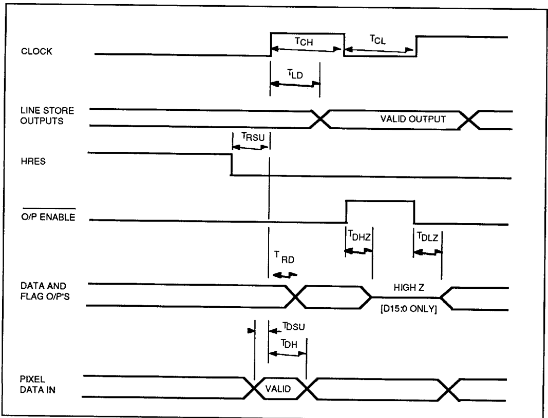
Fig. 10. I/O Timing
