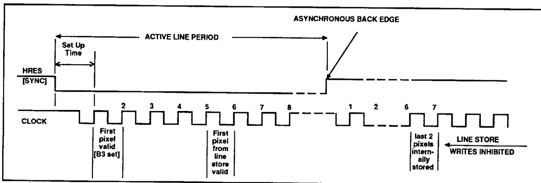
Fig.7 Pixel Input Delays
