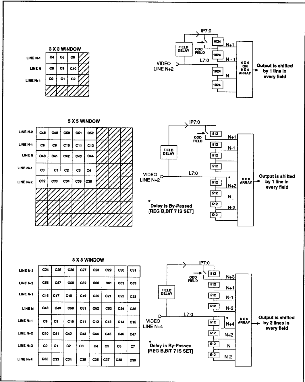
Figure 3. Line Delay Allocations in Single Device Interlaced Systems
