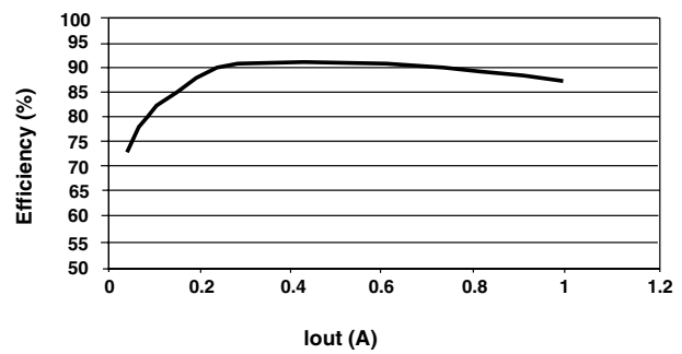
Efficiency Vs. Iout* Vin = 3.5V; Vout = 5.0V
