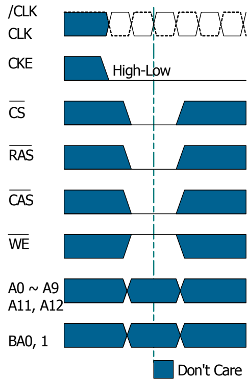
Self-Refresh Command
