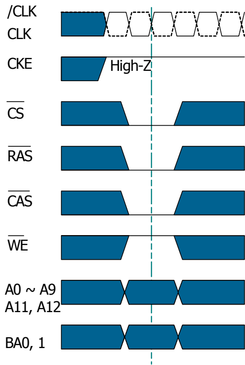
Auto-Refresh Command
