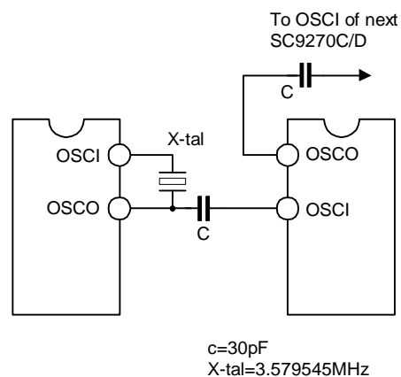
Figure 9 Oscillator Connection
