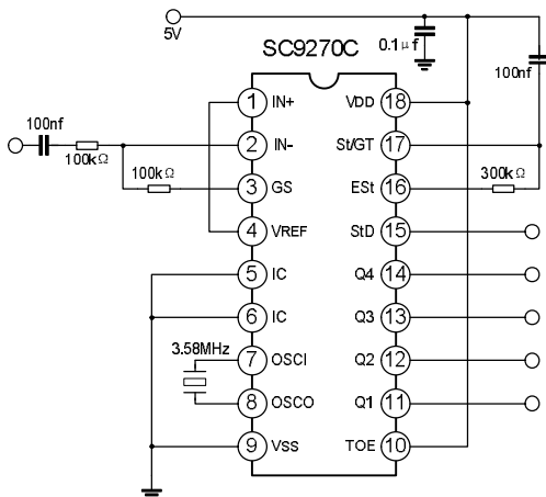
Figure 2. Single ended input configuration
