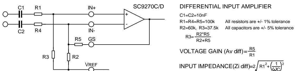
Figure 8. Differential input configuration
