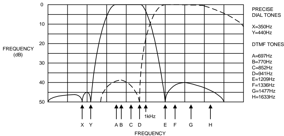
Figure 5. Filter Response
