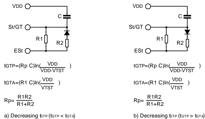
Figure 7. Guard time adjustment
