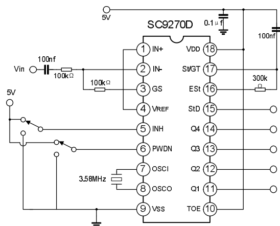
Figure 3. Single ended input configuration
