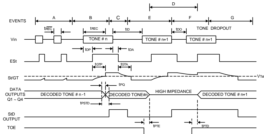
Figure 4. Timing diagram
