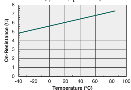
Typical On-Resistance vs. Temperature ( I_F=0\text{mA} , I_L=200\text{mA} )
