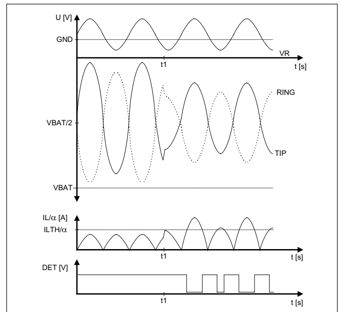
Figure 16. Off-hook during Ringing with an applied DC offset.
