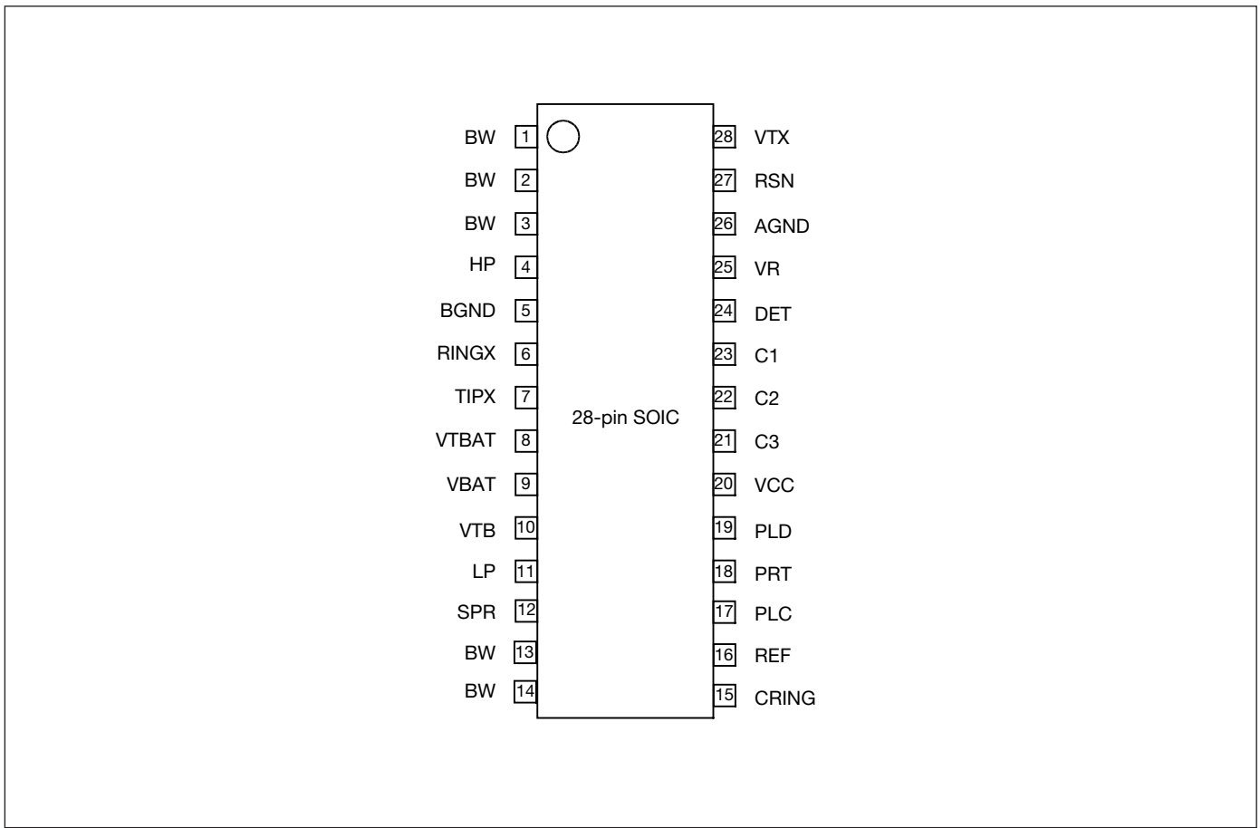
Figure 8. Pin configuration 28L-SOIC, top view.
