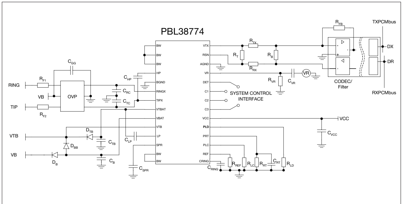
Figure 9. Single channel subscriber line interface with PBL 387 74/1 and Combo I type codec.
