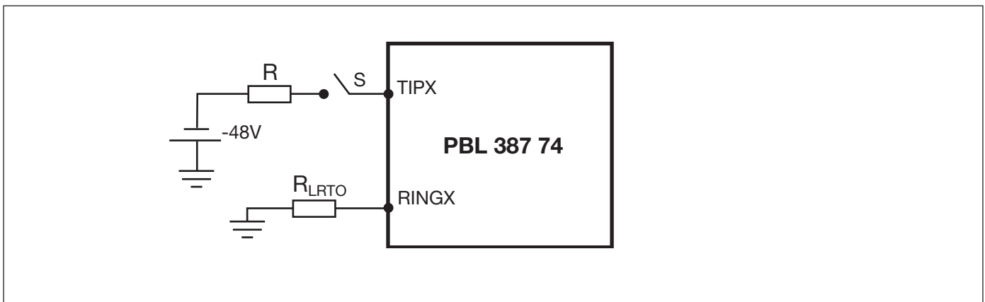
Figure 7. Tipx voltage.
