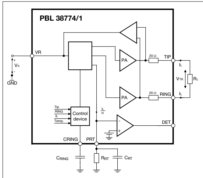
Figure 14. Ring loop schematic.
