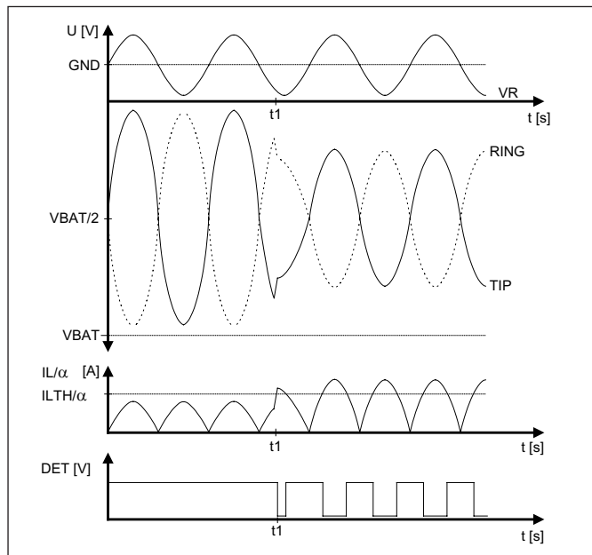
Figure 15. Off-hook during ringing.
