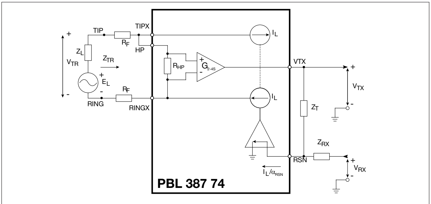
Figure 10. Simplified AC model of PBL 387 74/1.
