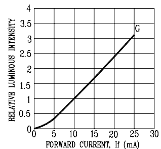
Fig3. Relative Luminous Intensity vs. DC Forward Current
