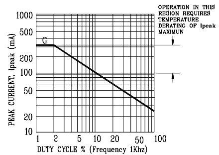
Fig5. Maximum Peak Current vs. Duty Cycle %
