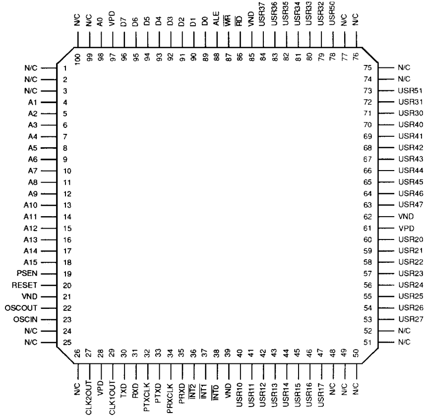
100-Lead TQFP
