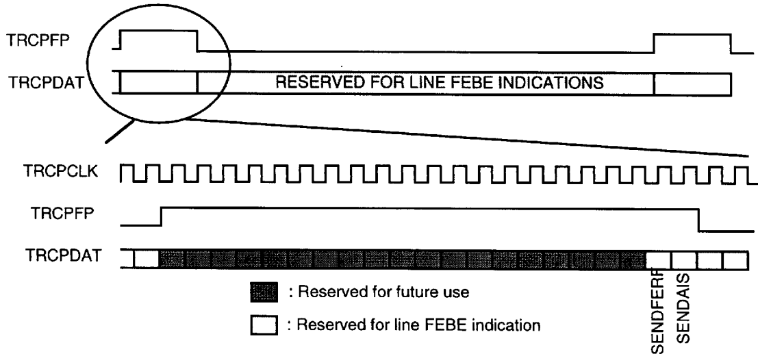
Fig. 23 Transmit Ring Control Port
