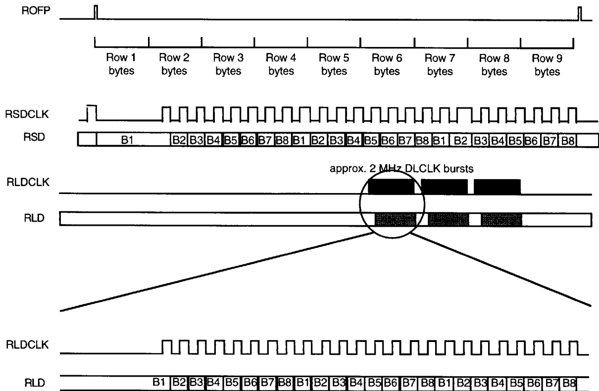
Fig. 19 Receive Data Link Clock and Data Alignment
