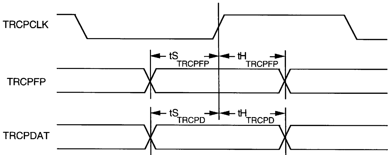
Fig. 31 Transmit Ring Control Port Input
