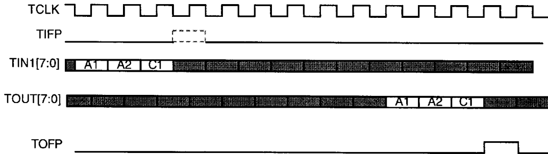
Fig. 3 STS-1 Byte Serial Transmit Frame Pulse and Data Alignment
