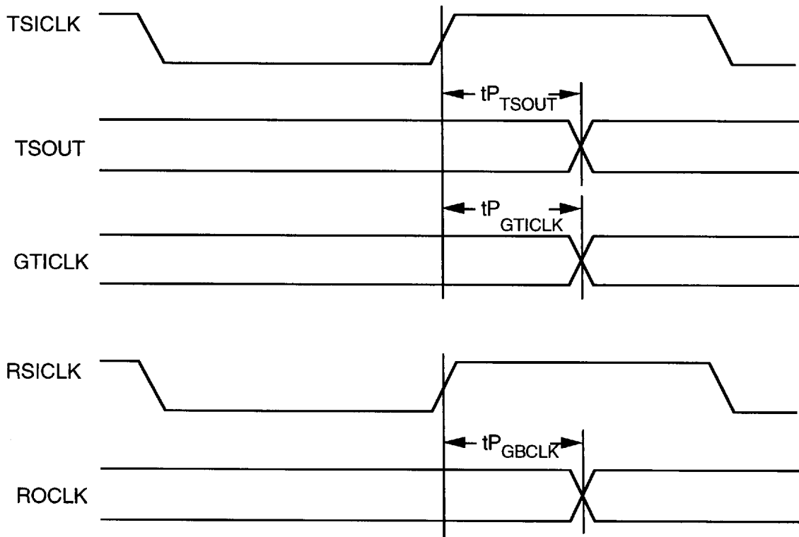
Fig. 35 STS-1 Output Timing
