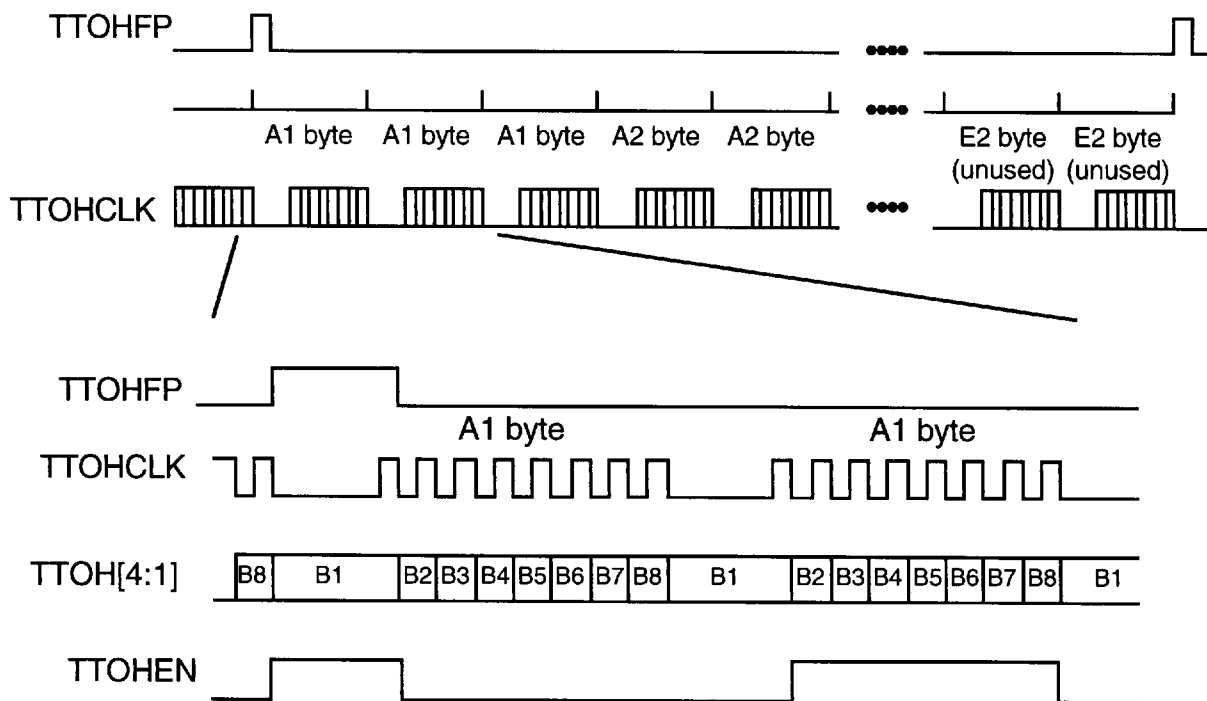
Fig. 22 Transport Overhead Insertion
