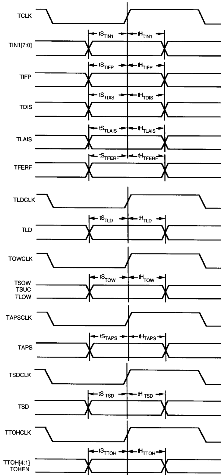
Fig. 28 Transmit Input Timing with BIMX Bypassed
