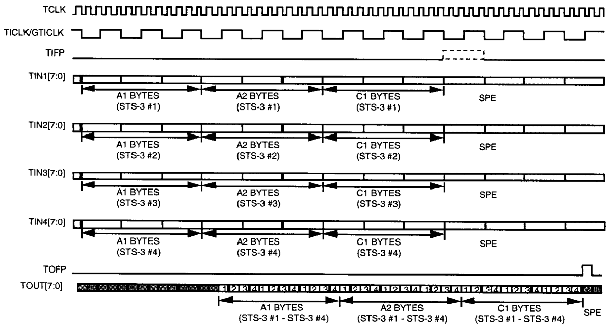
Fig. 4 Byte Interleaved Multiplex Frame Pulse and Data Alignment
