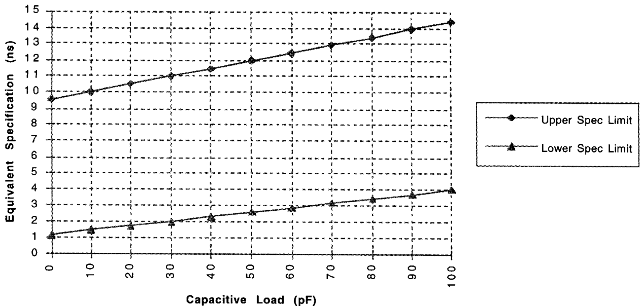
Equivalent Specification for tPTOUT
