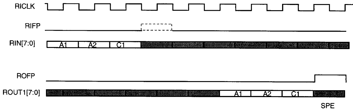
Fig. 7 STS-1 Byte Serial Receive Frame Pulse and Data Alignment
