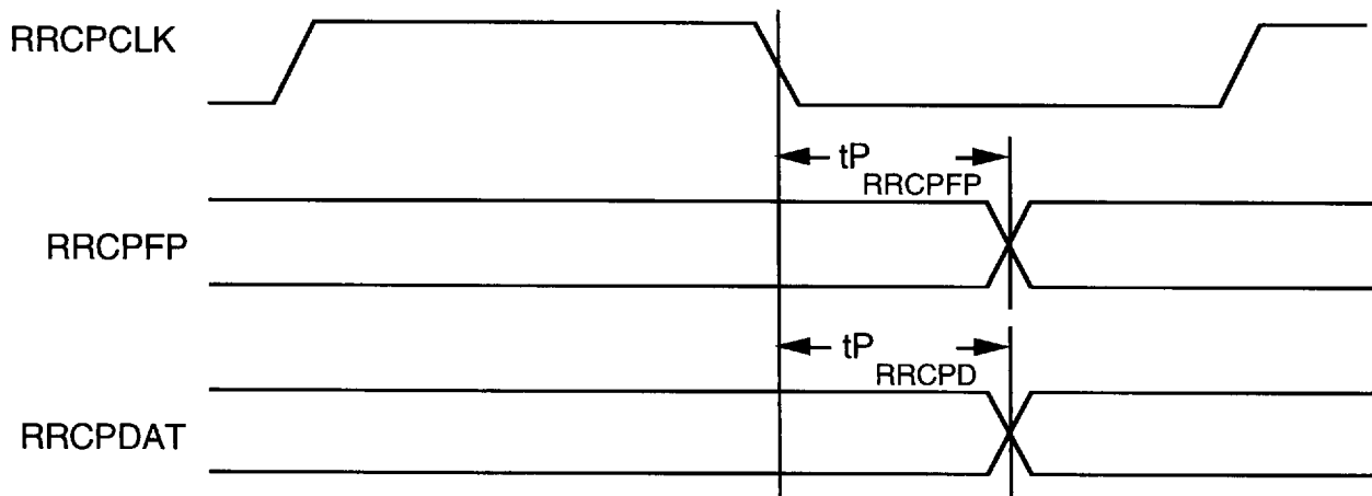
Fig. 36 Ring Control Port Output
