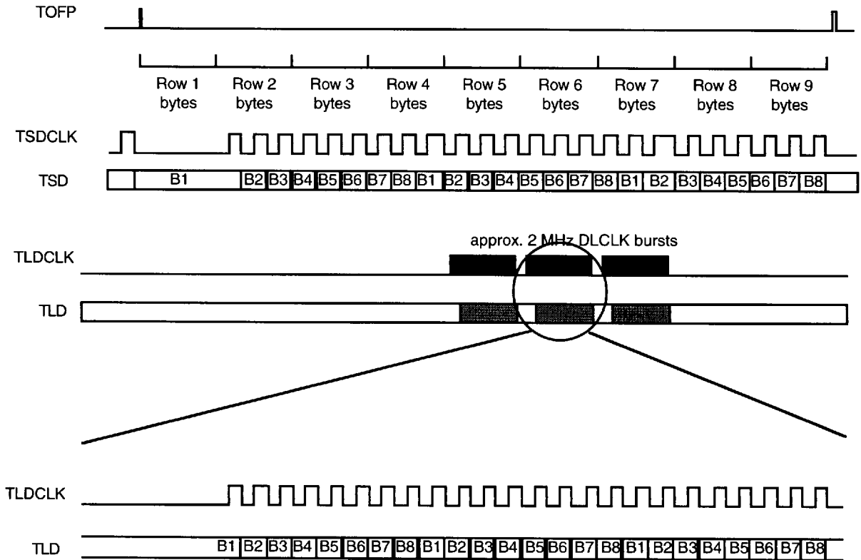
Fig. 18 Transmit Data Link Clock and Data Alignment
