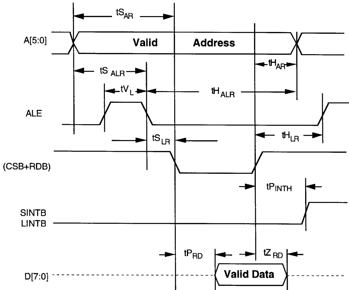
Fig. 25 Microprocessor Interface Read Access Timing
