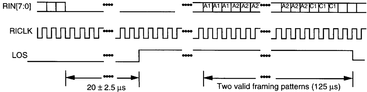
Fig. 13 Loss of Signal Declaration/Removal
