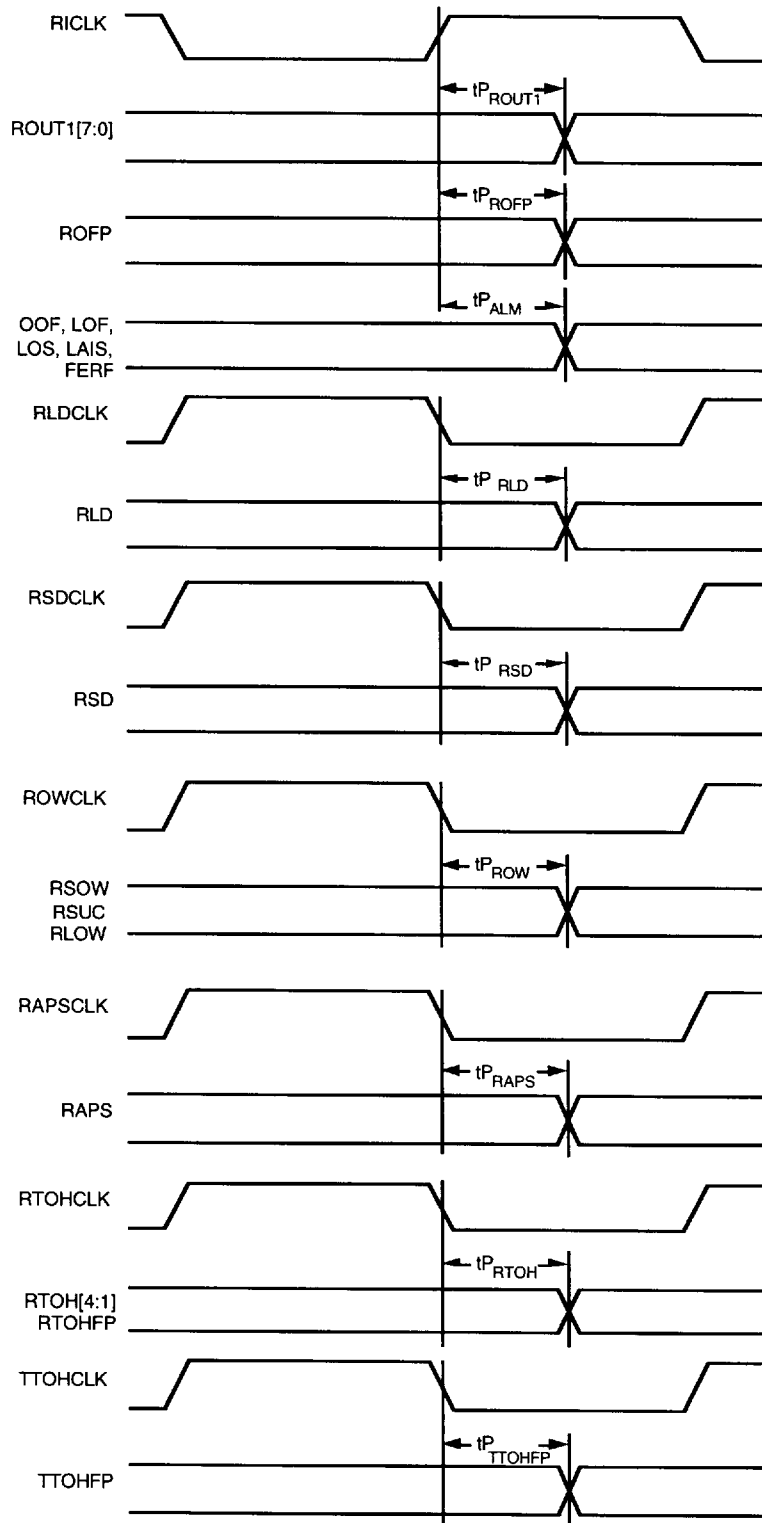
Fig. 32 Receive Output Timing with BIDX Bypassed
