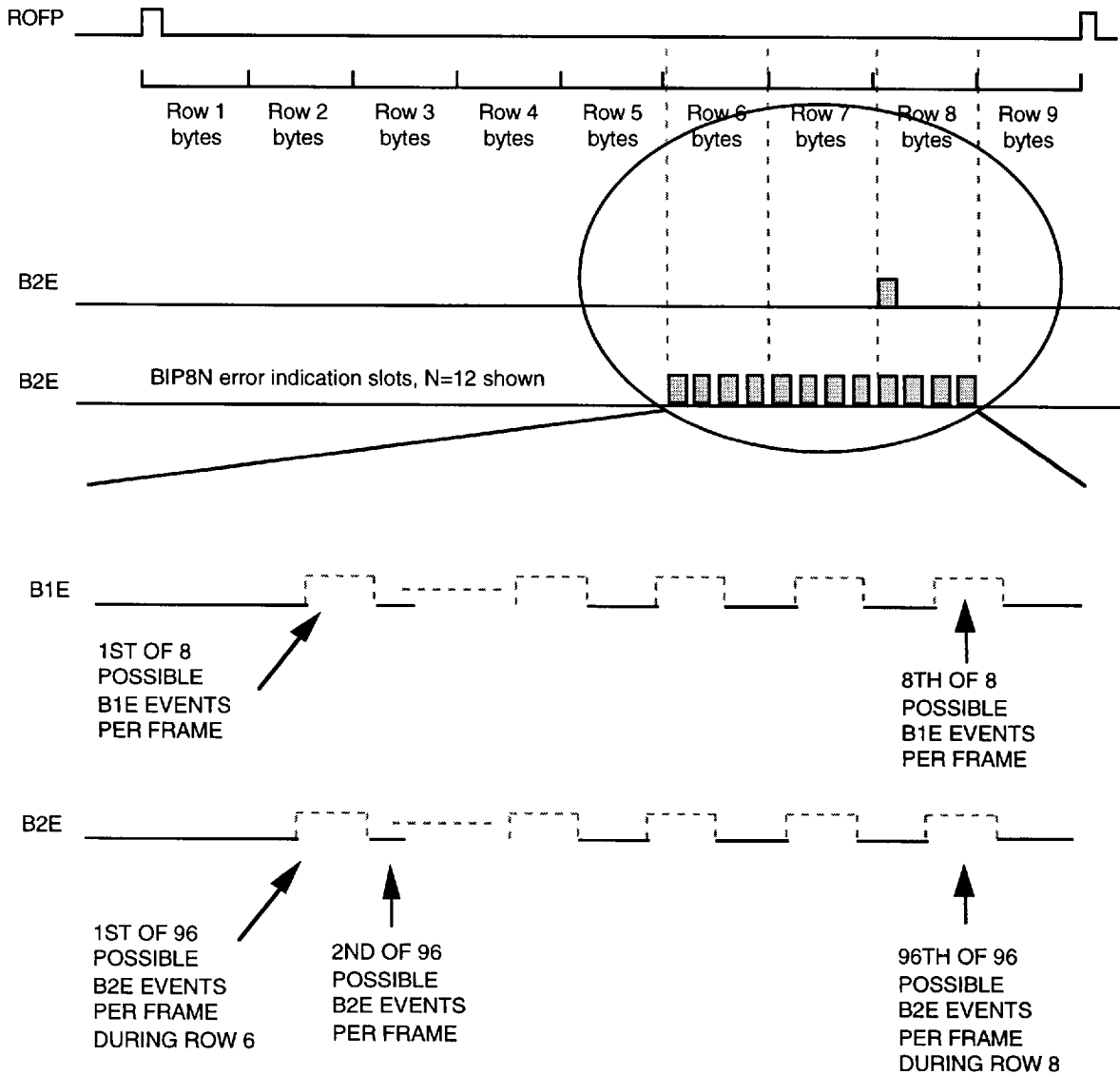
Fig. 20 B1 and B2 Error Event Occurrence
