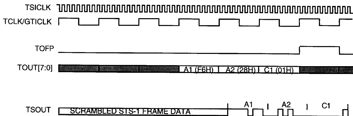
Fig. 2 STS-1 Bit Serial Transmit Frame Pulse and Data Alignment
