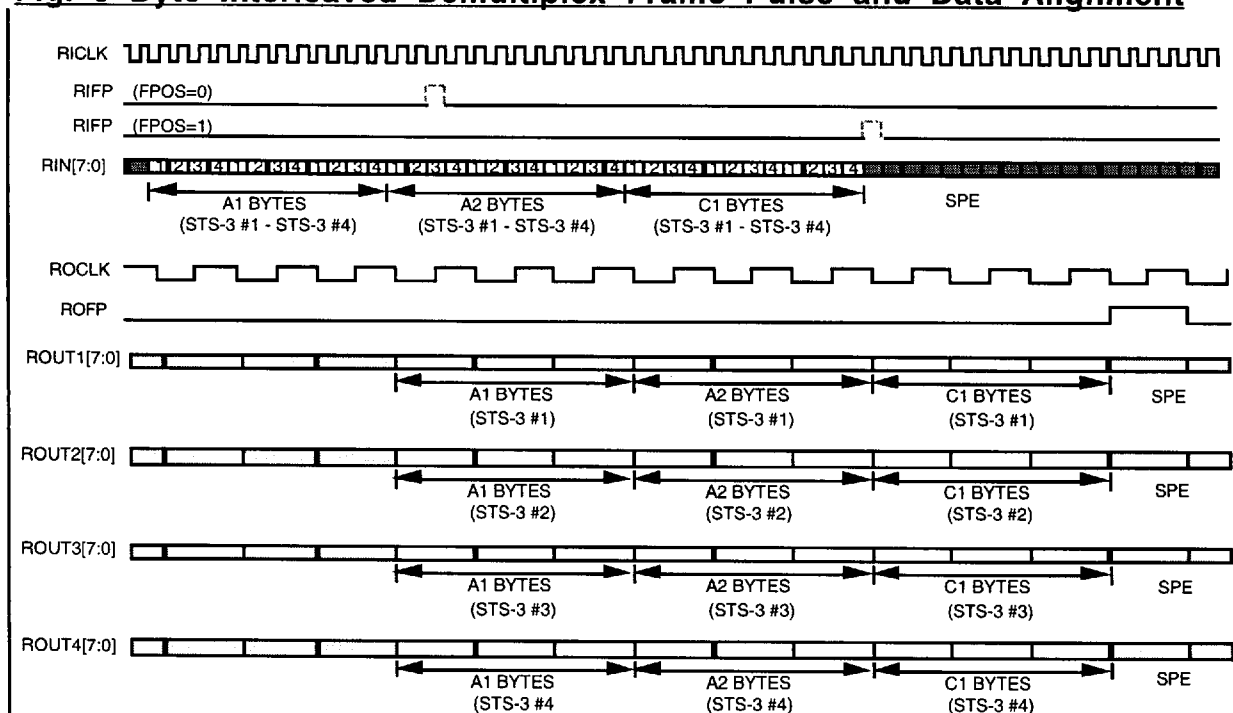
Fig. 8 Byte Interleaved Demultiplex Frame Pulse and Data Alignment
