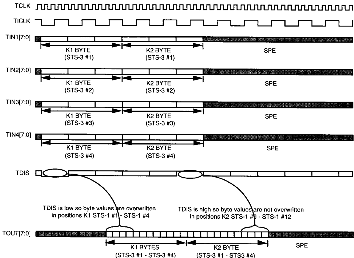
Fig. 10 Transport Overhead Overwrite Enable and Disable with Multiplexing Enabled
