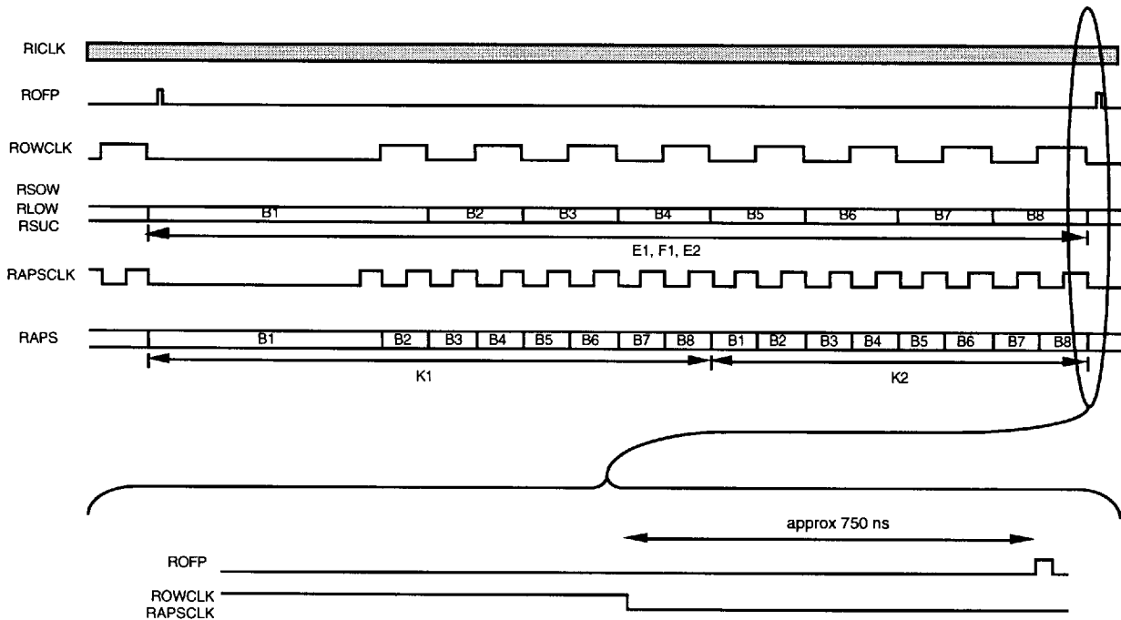
Fig. 17 Receive Overhead Clock and Data Alignment
