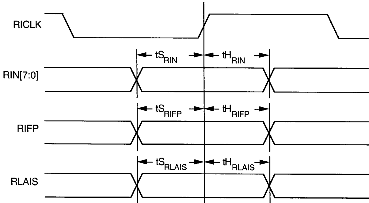
Fig. 27 Receive Input Timing
