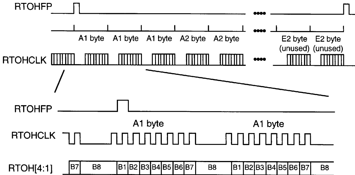
Fig. 21 Transport Overhead Extraction
