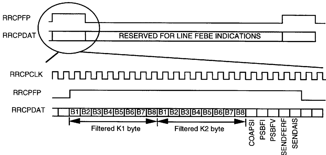
Fig. 24 Receive Ring Control Port
