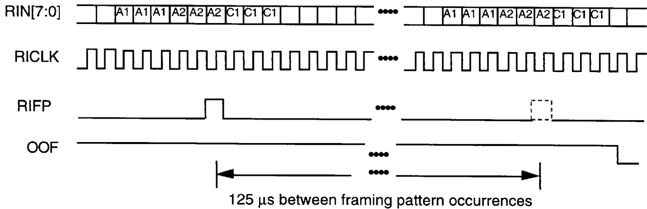
Fig. 11 In Frame Declaration
