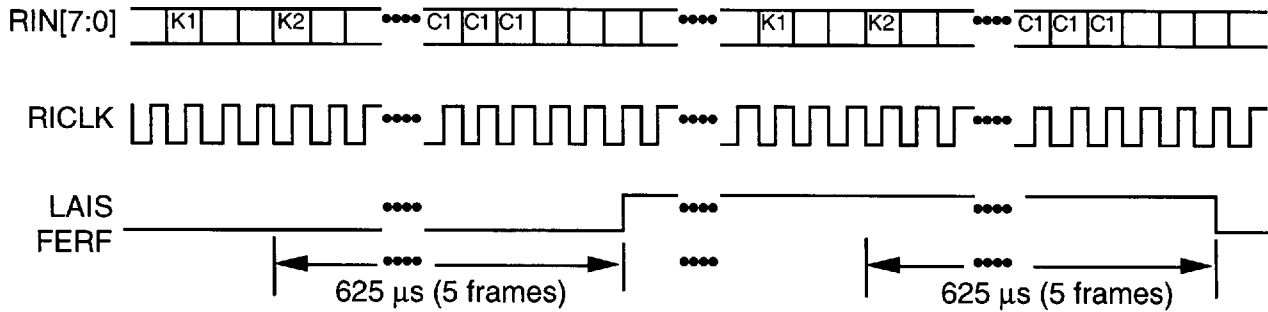
Fig. 15 Line AIS and Line FERF Declaration/Removal
