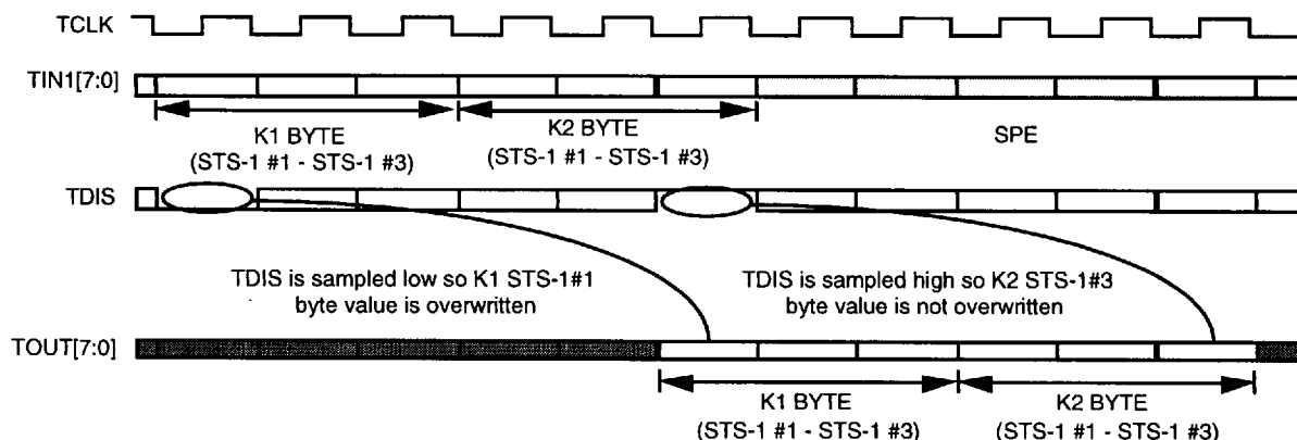
Fig. 9 Transport Overhead Overwrite Enable and Disable with Multiplexing Bypassed
