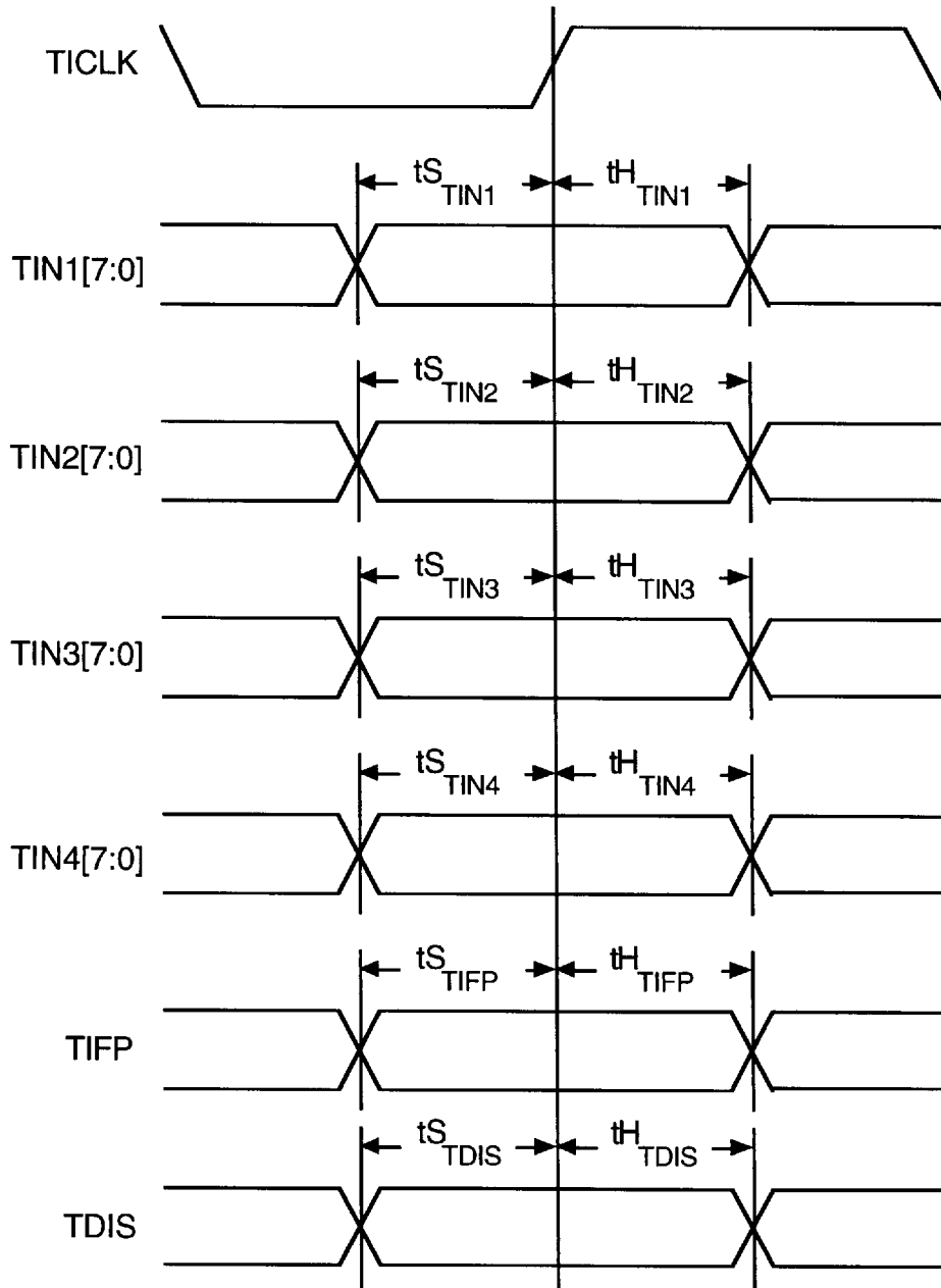
Fig. 29 Transmit Input Timing to BIMX
