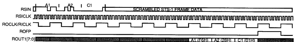
Fig. 6 STS-1 Bit Serial Receive Frame Pulse and Data Alignment
