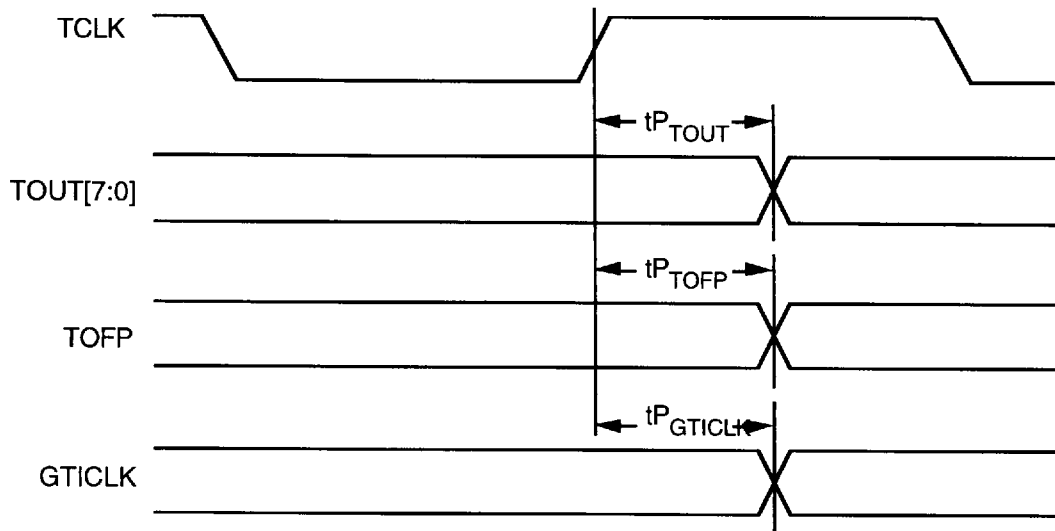
Fig. 34 Transmit Output Timing
