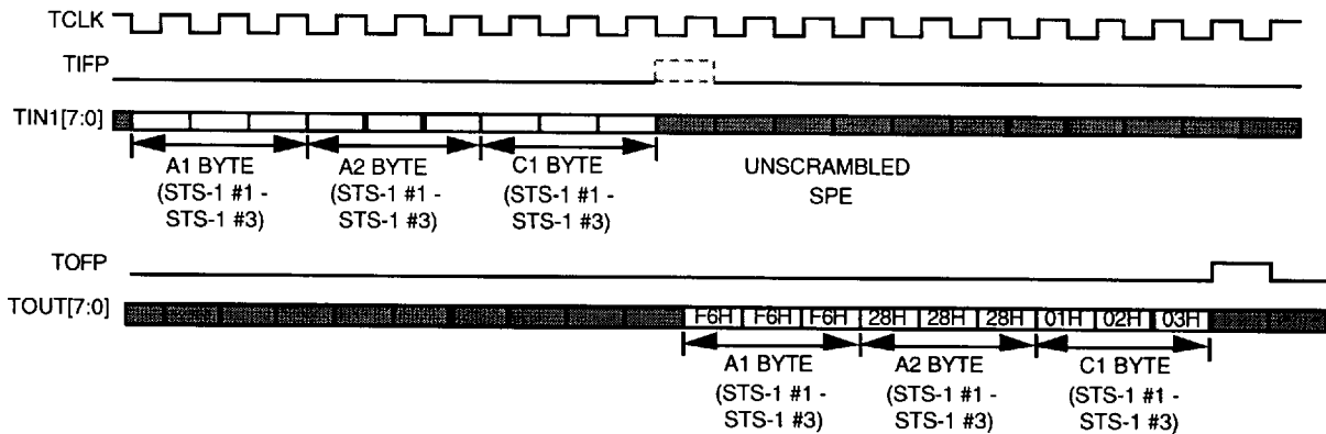
Fig. 1 STS-3 Transmit Frame Pulse and Data Alignment
