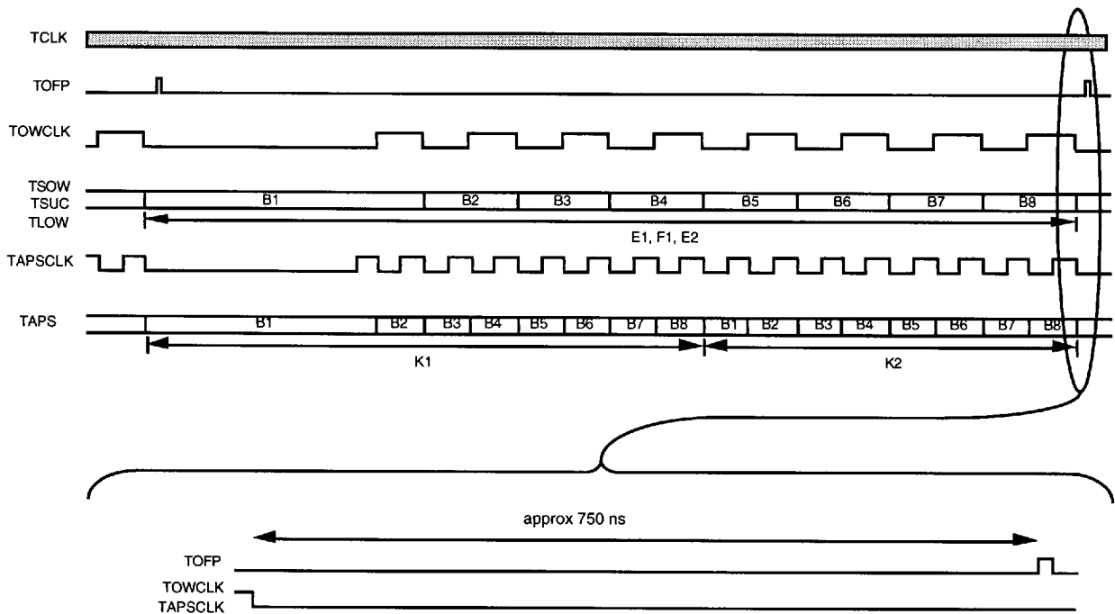
Fig. 16 Transmit Overhead Clock and Data Alignment
