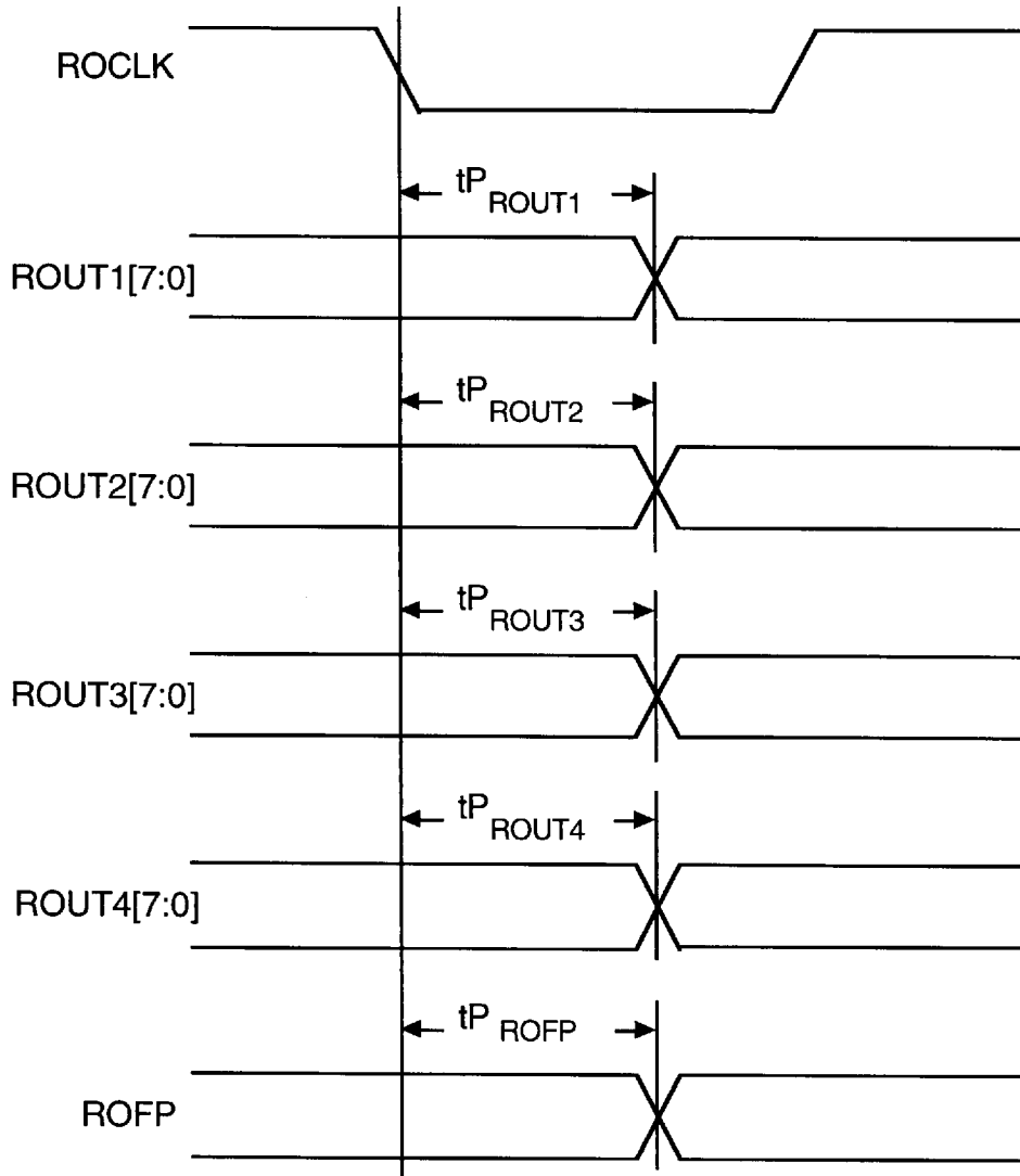
Fig. 33 Receive Output Timing of BIDX
