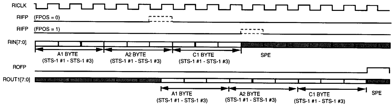
Fig. 5 STS-3 Receive Frame Pulse and Data Alignment
