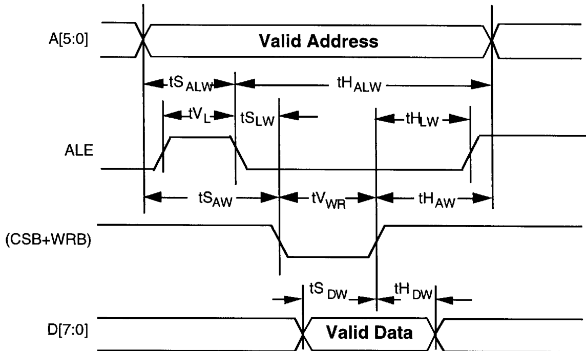
Fig. 26 Microprocessor Interface Write Access Timing
