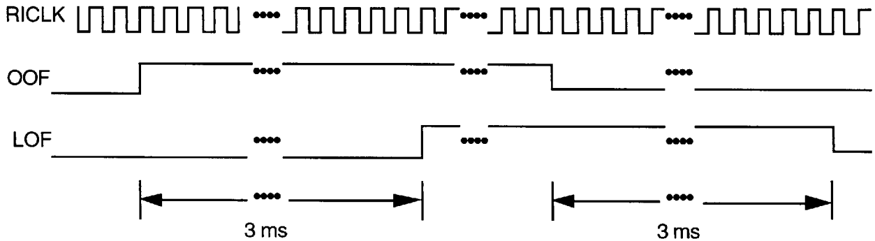
Fig. 14 Loss of Frame Declaration/Removal
