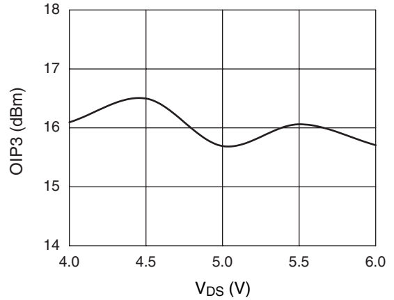
Two-Tone Output Third-Order Intercept @ 38 GHz
