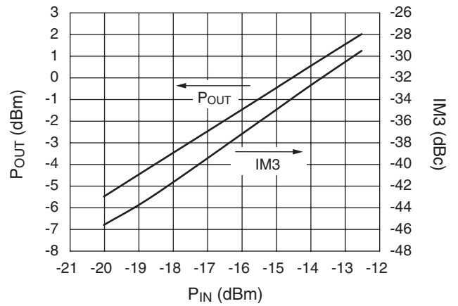
Output Power and Relative Third-Order Intermodulation Products F = 38\text{ GHz}, V_{DS} = 5\text{ V}
