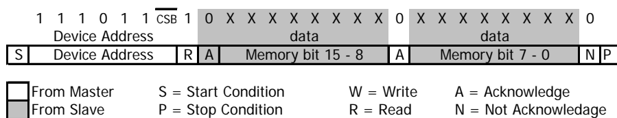
Figure 12: I 2 C answer from MS5607-02BA
