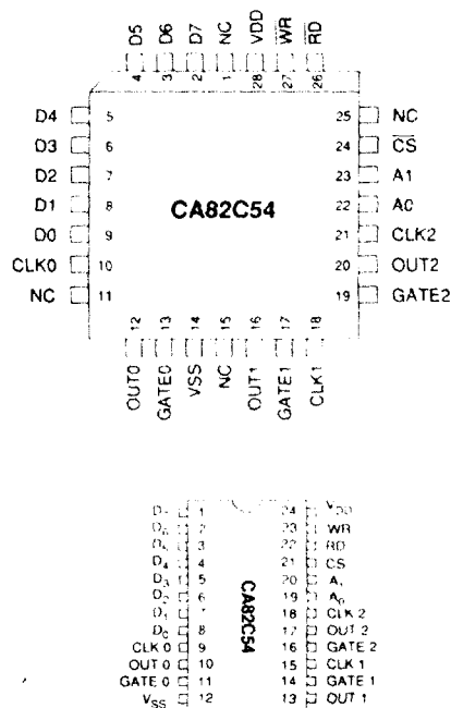
Figure 2 : PLCC and DIP PIN CONFIGURATIONS
