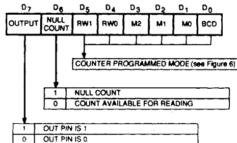
Figure 11 : STATUS BYTE
