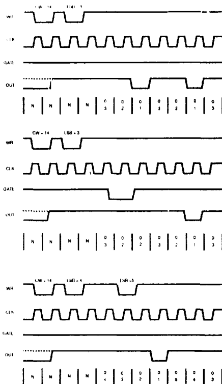
Figure 15 : MODE 2 TIMING
