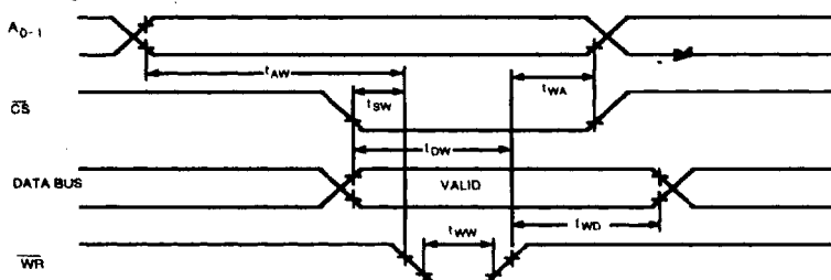
Figure 4 : TIMING DIAGRAMS
