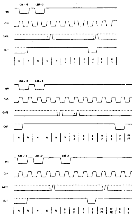
Figure 18 : MODE 5 TIMING
