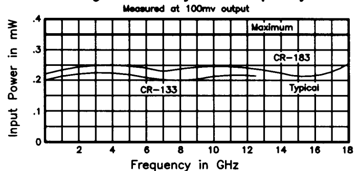
High Sensitivity Vs. Frequency
