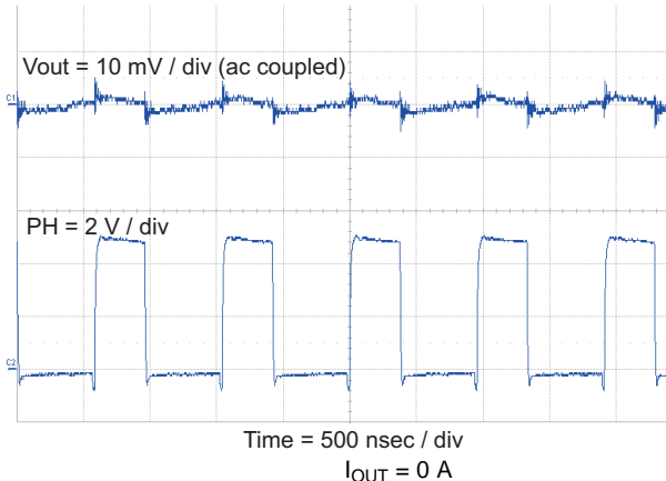
Figure 45. Output Ripple
