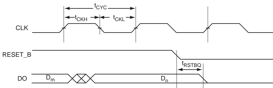
Figure 2-29 • RAM Reset
