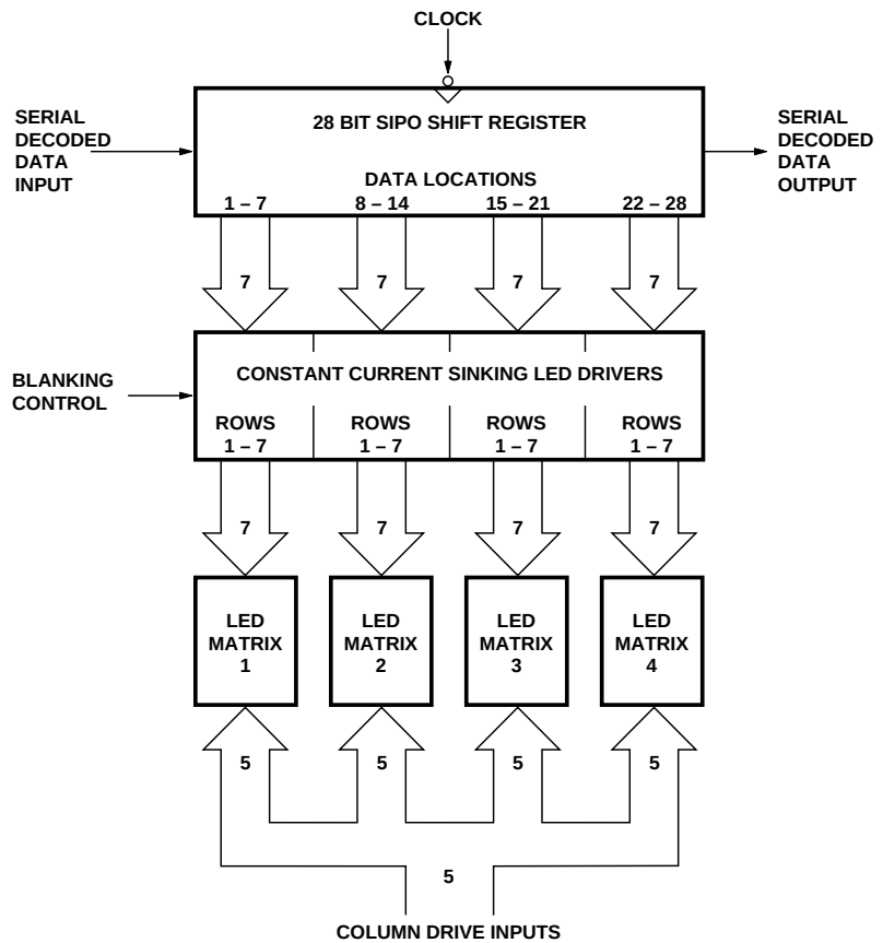
Figure 5. Block Diagram of HDSP-2301/-2302/-2303.
