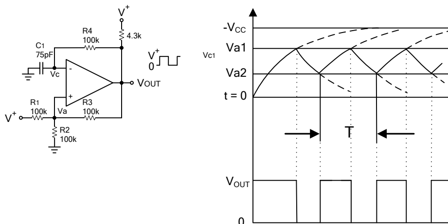
Squarewave Oscillator
