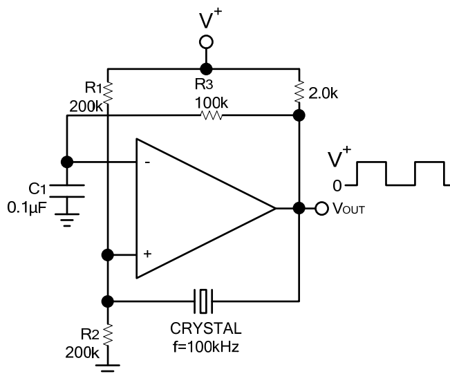
Crystal controlled Oscillator
