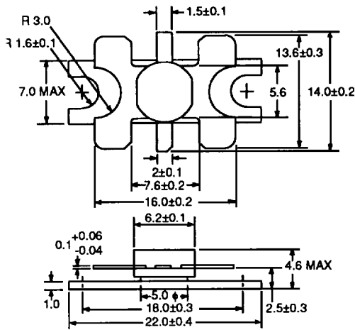
PACKAGE OUTLINE 90
