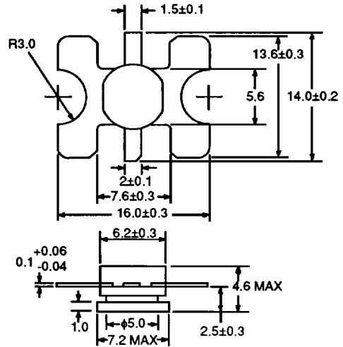
PACKAGE OUTLINE 91
