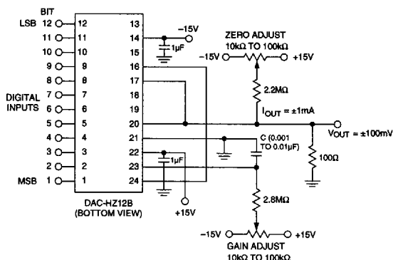
Figure 6. Bipolar Current Output Connections
