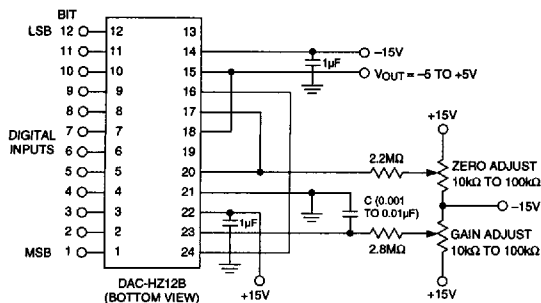
Figure 5. Bipolar Voltage Output Connections
