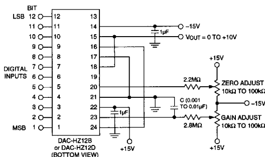
Figure 2. Unipolar Voltage Output Connections
