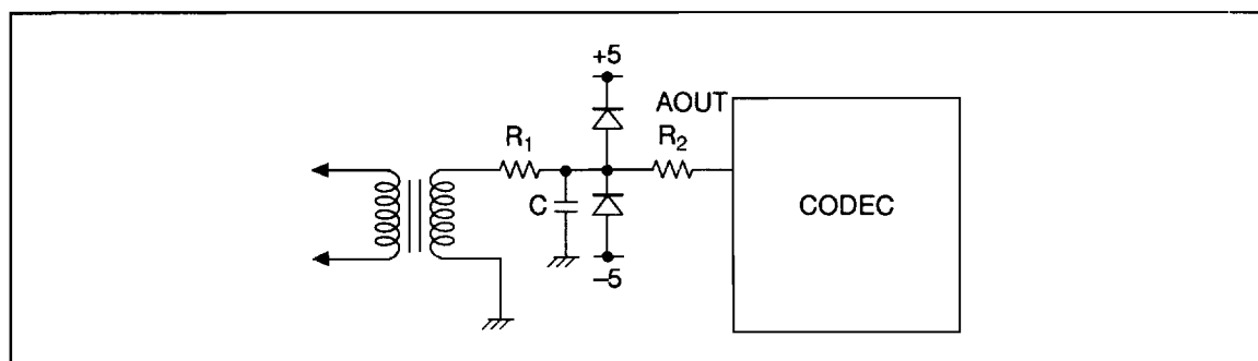
Figure 3 Surge Prevention Circuit
