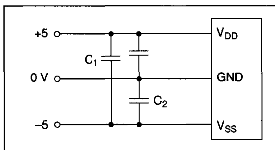
Figure 2 Bypass Capacitors
