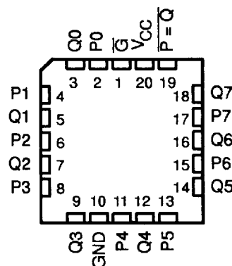
SN54ALS688 ... FK PACKAGE (TOP VIEW)
