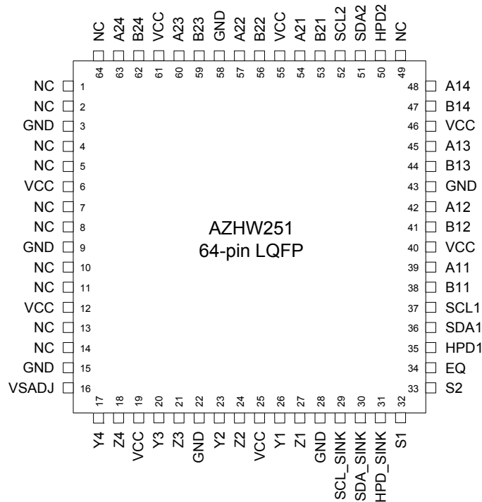
Pin Configuration
