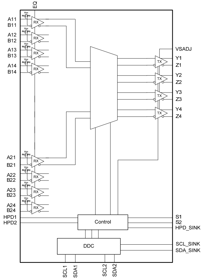
Circuit diagram
