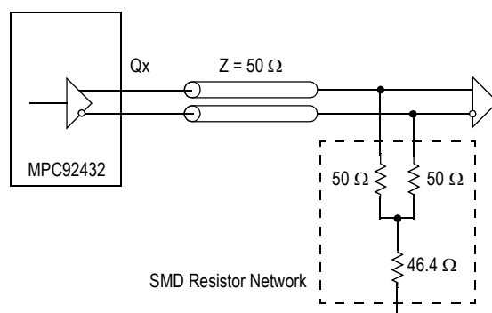
Figure 12. Resistor Network Termination
