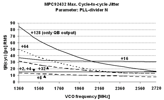
Figure 8. MPC92432 Cycle-to-Cycle Jitter
