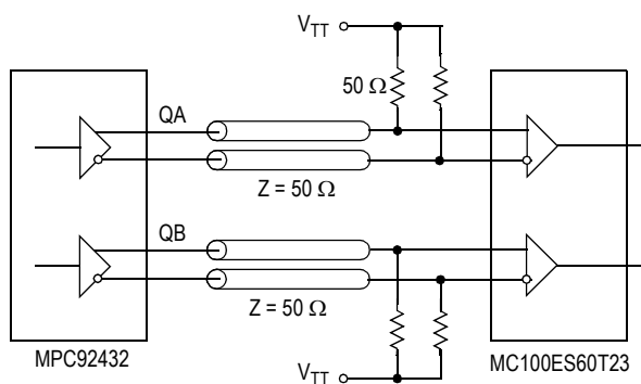
Figure 13. Interfacing with LVCMOS Logic for Frequency < 180 MHz
