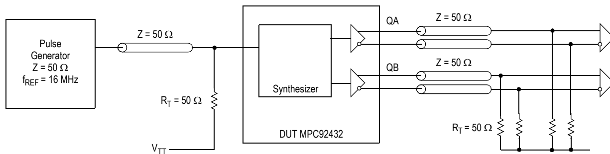
Figure 10. MPC92432 AC Test Reference
