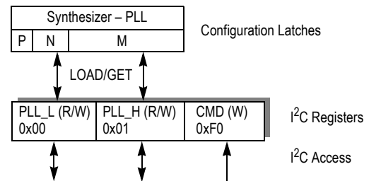
Figure 3. I 2 C Mode Register Set
