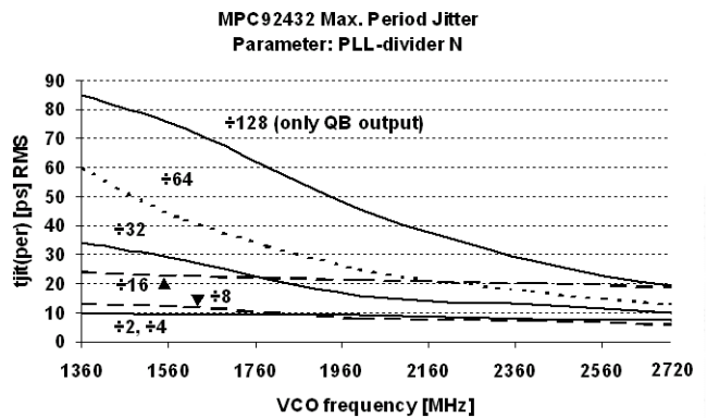
Figure 9. MPC92432 Period Jitter
