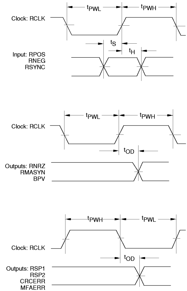
Figure 13. RCLK Input/Output Timing
