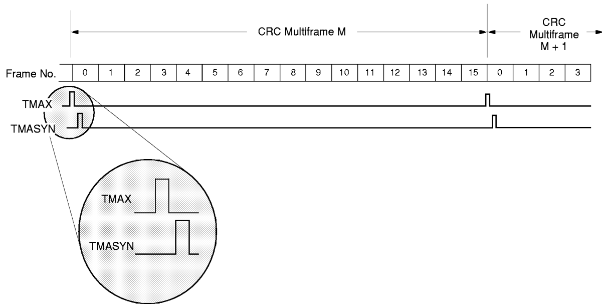
Figure 6. Transmit CRC Multiframe-Bt8070 Mode 256S.
