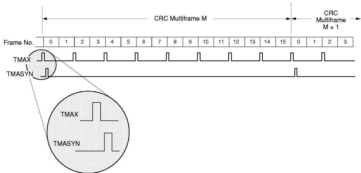
Figure 7. Transmit CRC Multiframe-Bt8070 Mode 256N
