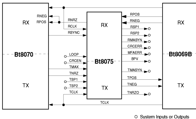
Figure 1. Bt8075 Functional Interface
