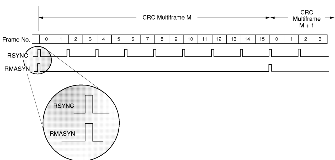
Figure 10. Receive CRC Multiframe-Bt8070 Mode 256N
