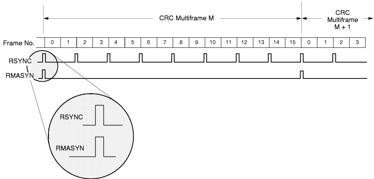
Figure 9. Receive CRC Multiframe-Bt8070 Mode 256S
