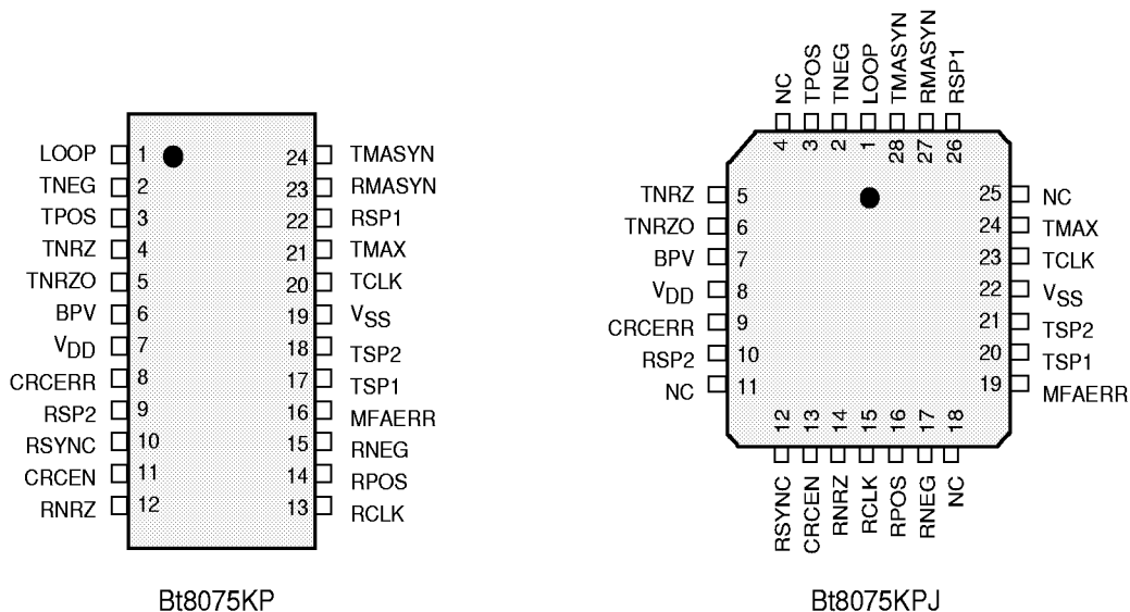
Figure 3. Bt8075 Pin Assignments
