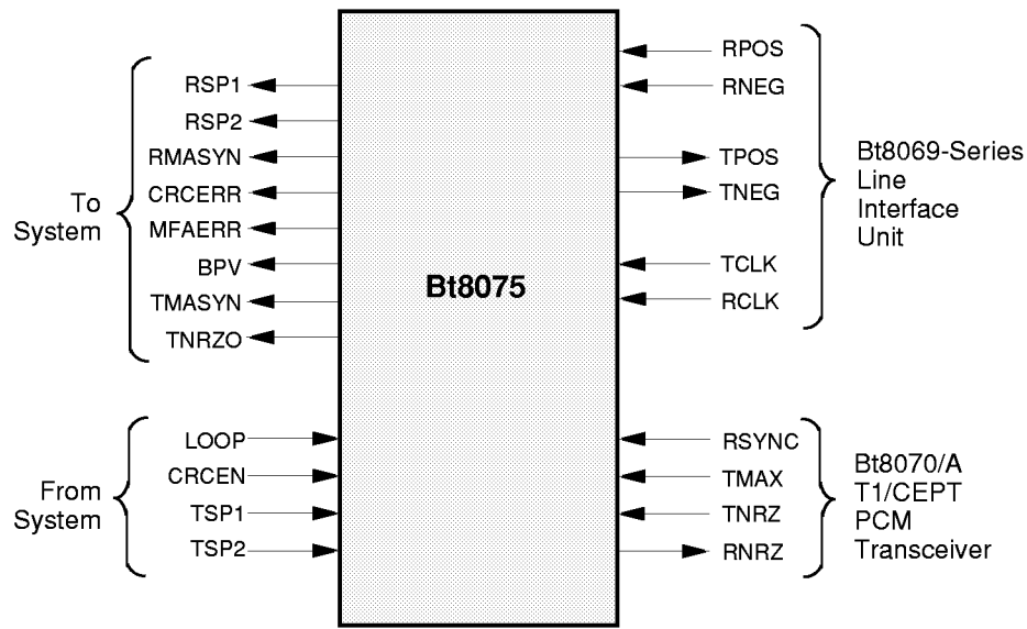
Figure 2. Bt8075 Interface Signals
