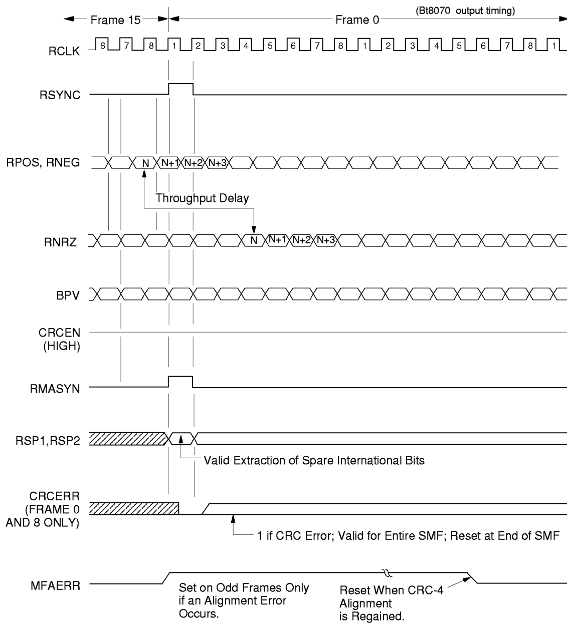
Figure 11. Bt8075 Receive Timing
