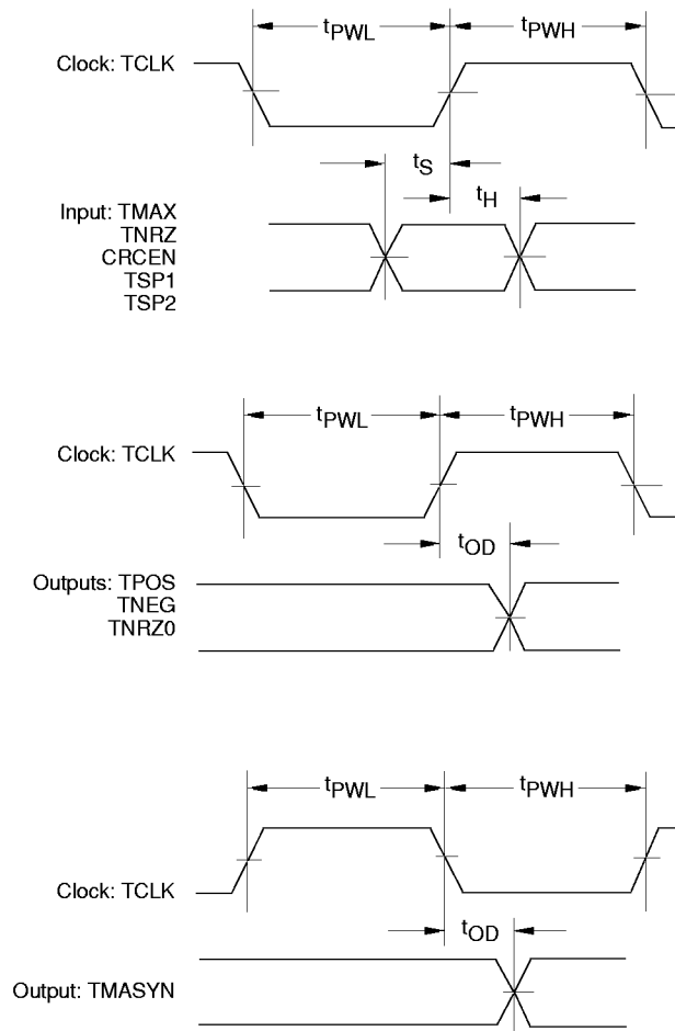
Figure 12. TCLK Input/Output Timing
