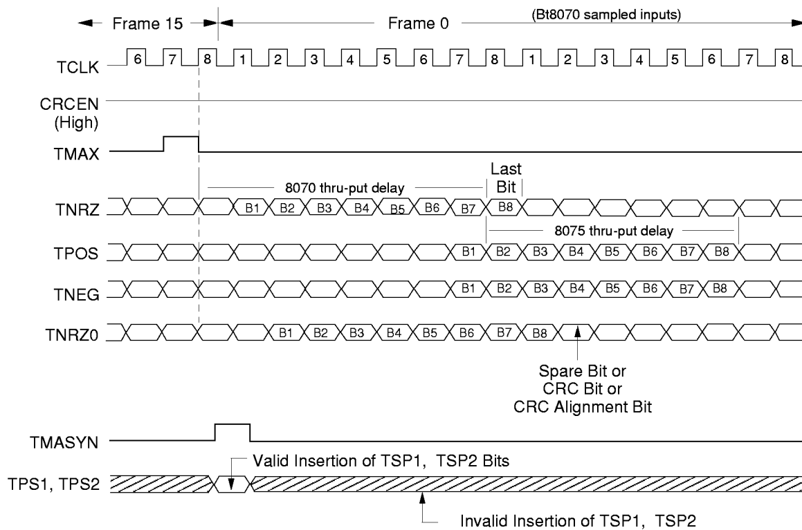
Figure 5. Bt8075 Transmit Timing
