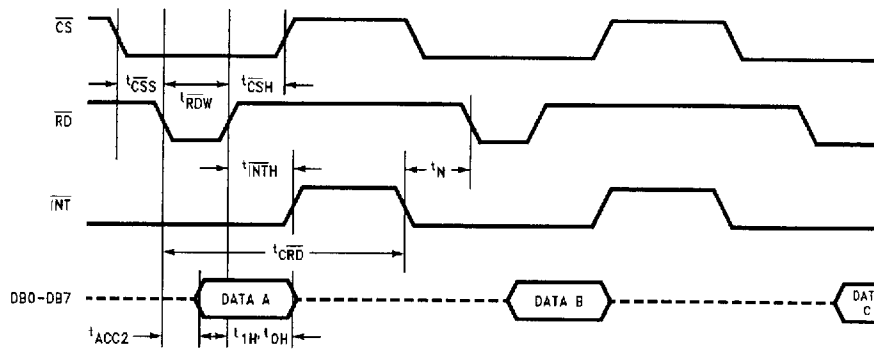
FIGURE 4. \overline{RD} Mode (Pipeline Operation); t_{RDW} must be between 200 ns and 400 ns. (Mode Pin is Low)
