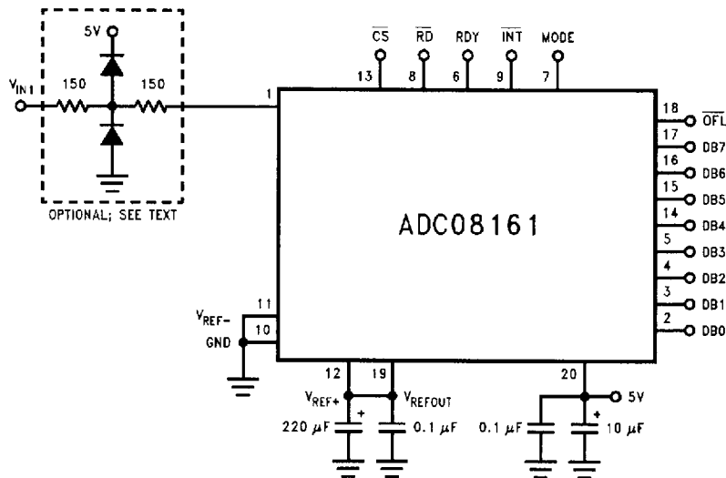
FIGURE 7. Analog Input Options
