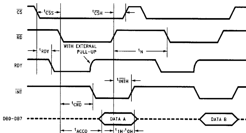
FIGURE 1. \overline{RD} Mode (Mode Pin is Low)
