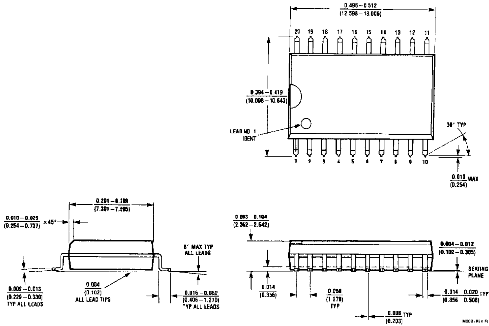
Wide-Body Small-Outline Order Number ADC08161BIWM or ADC08161CIWM NS Package Number M20B
