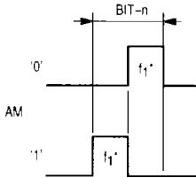
Figure 1. Signal Coding
