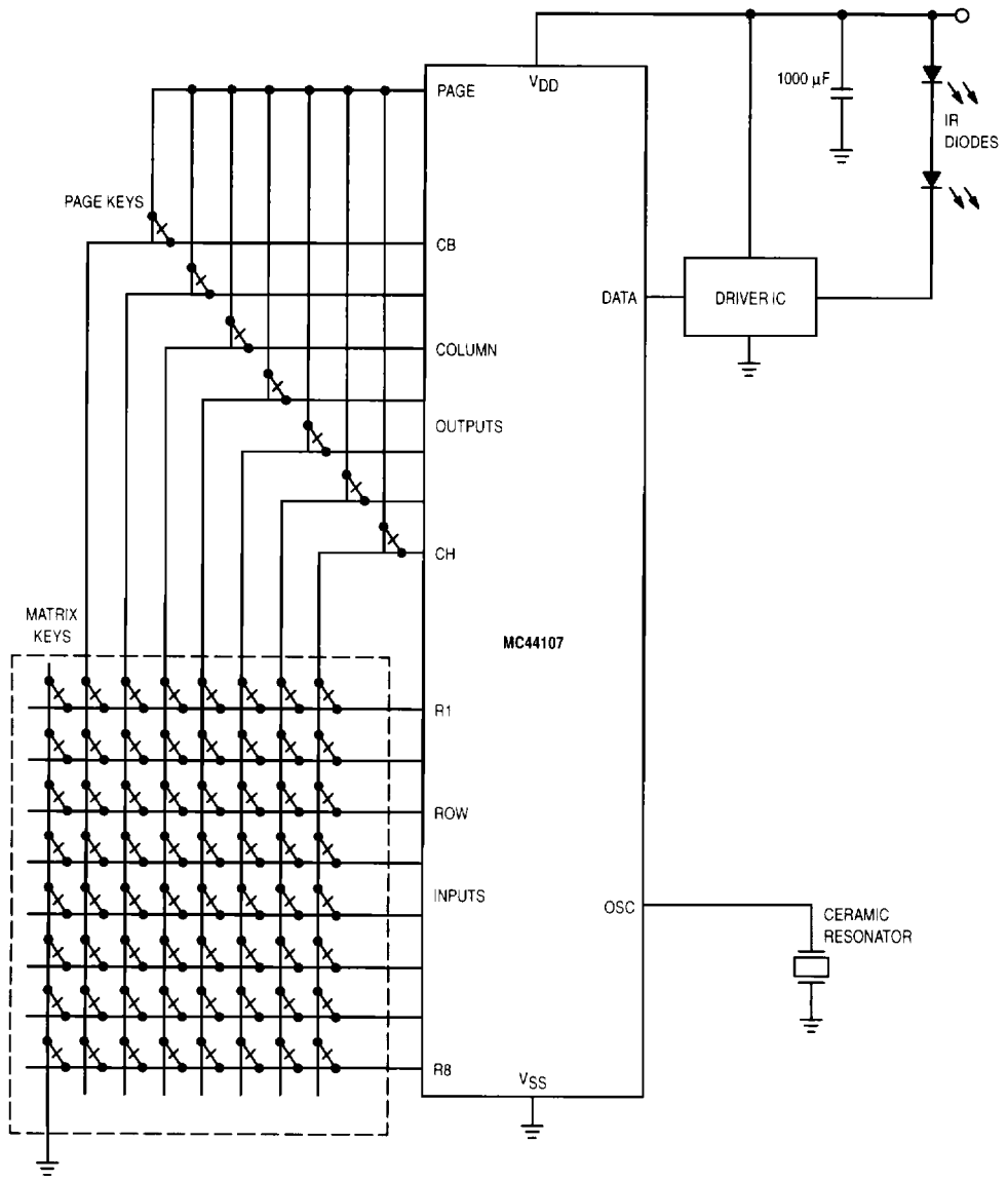
Figure 3. Transmitter Circuit
