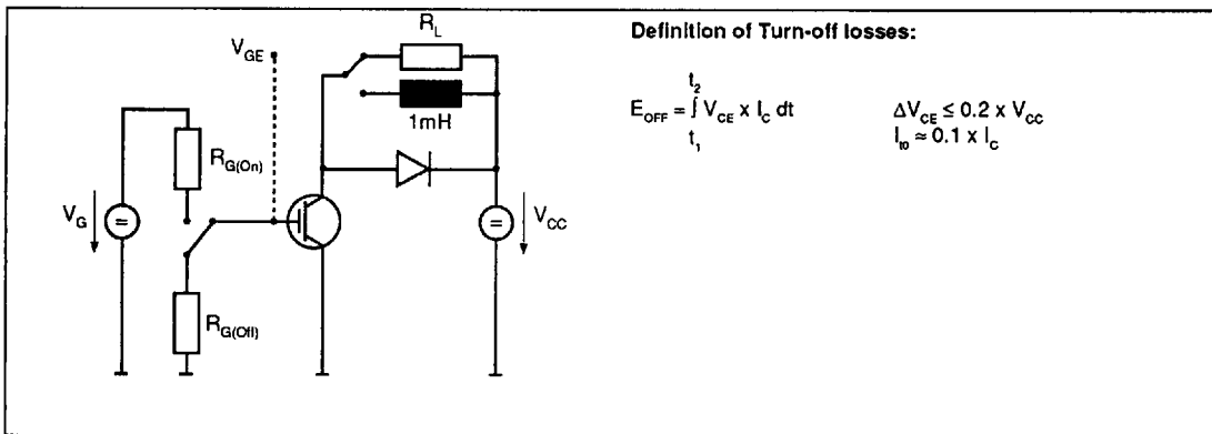
Fig.3 Test circuit
