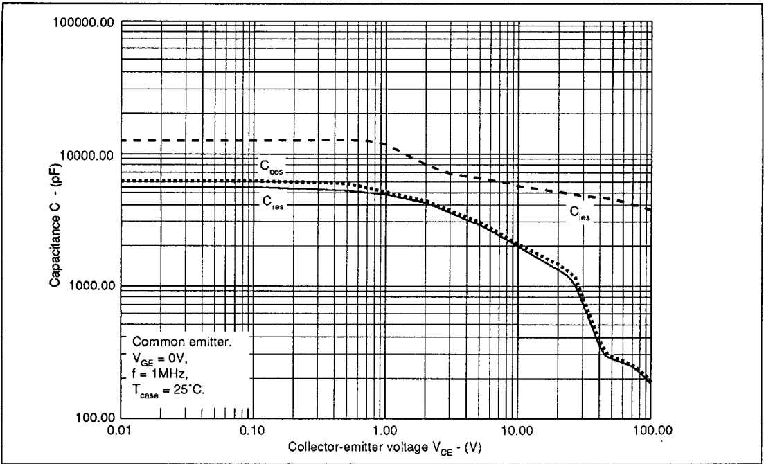
Fig.12 Typical capacitance
