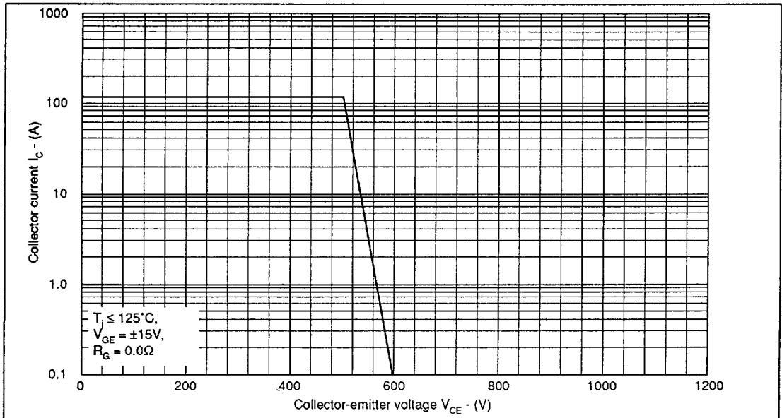
Fig.13 Reverse bias safe operating area
