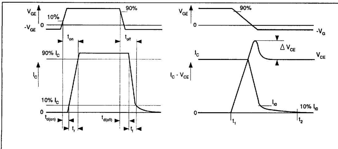
Fig.4 Definition of switching times
