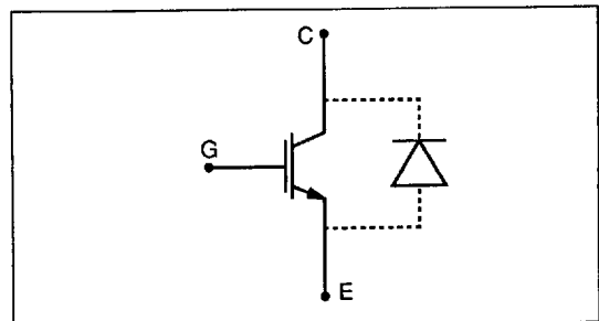
Fig.2 ITE60X06 circuit
