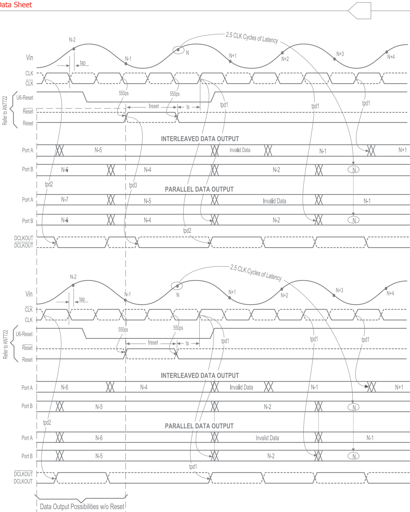
Figure 2. Dual Mode Timing Diagram
