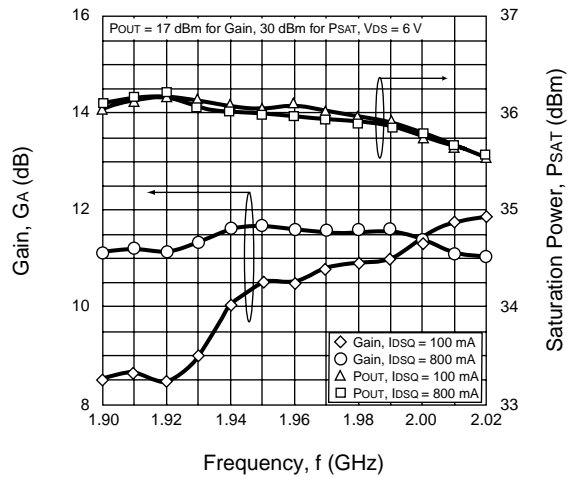
GAIN AND SATURATION POWER vs. FREQUENCY
