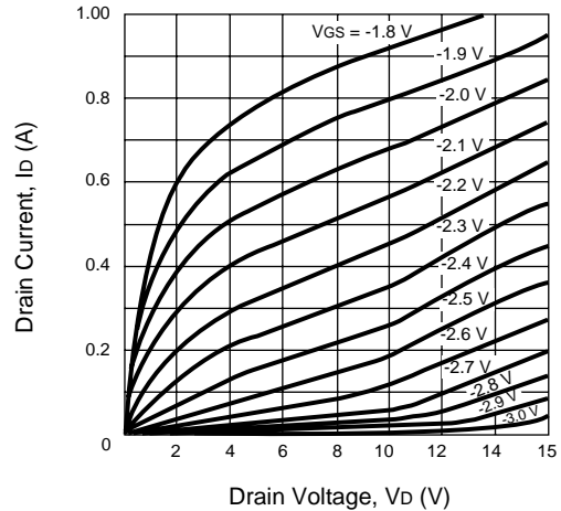
DRAIN CURRENT vs. DRAIN VOLTAGE
