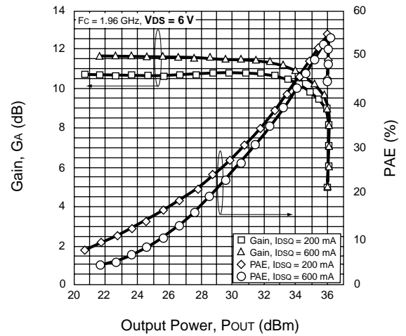
GAIN AND PAE vs. OUTPUT POWER
