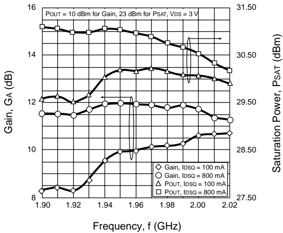
GAIN AND SATURATION POWER vs. FREQUENCY
