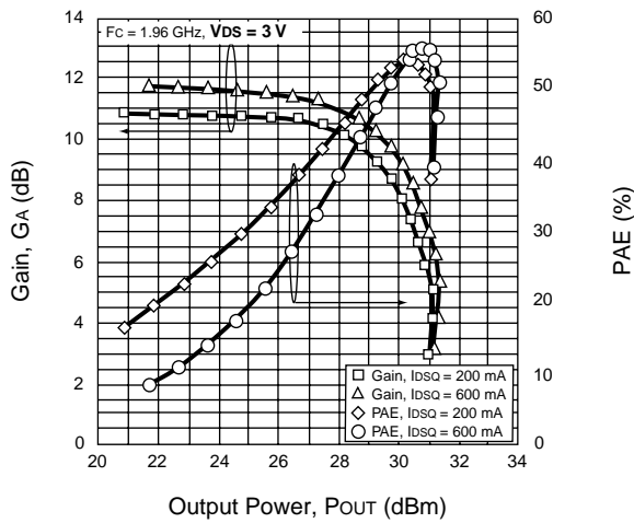
GAIN AND PAE vs. OUTPUT POWER
