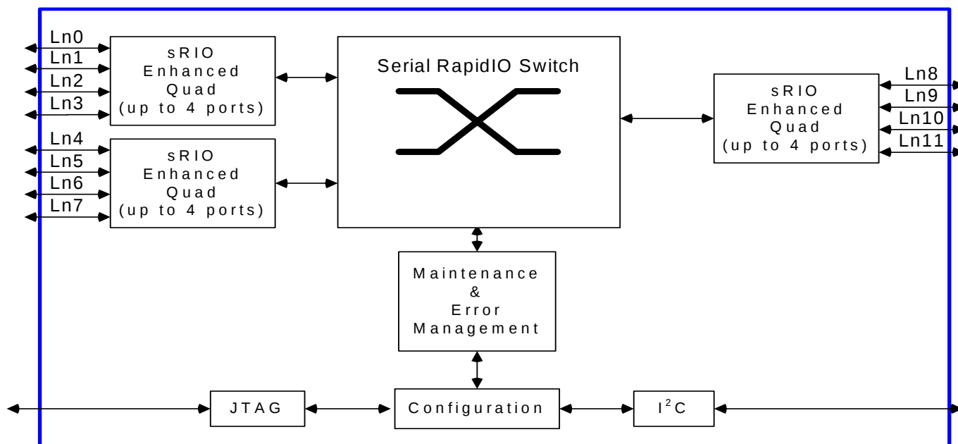
Figure 1 Block diagram
