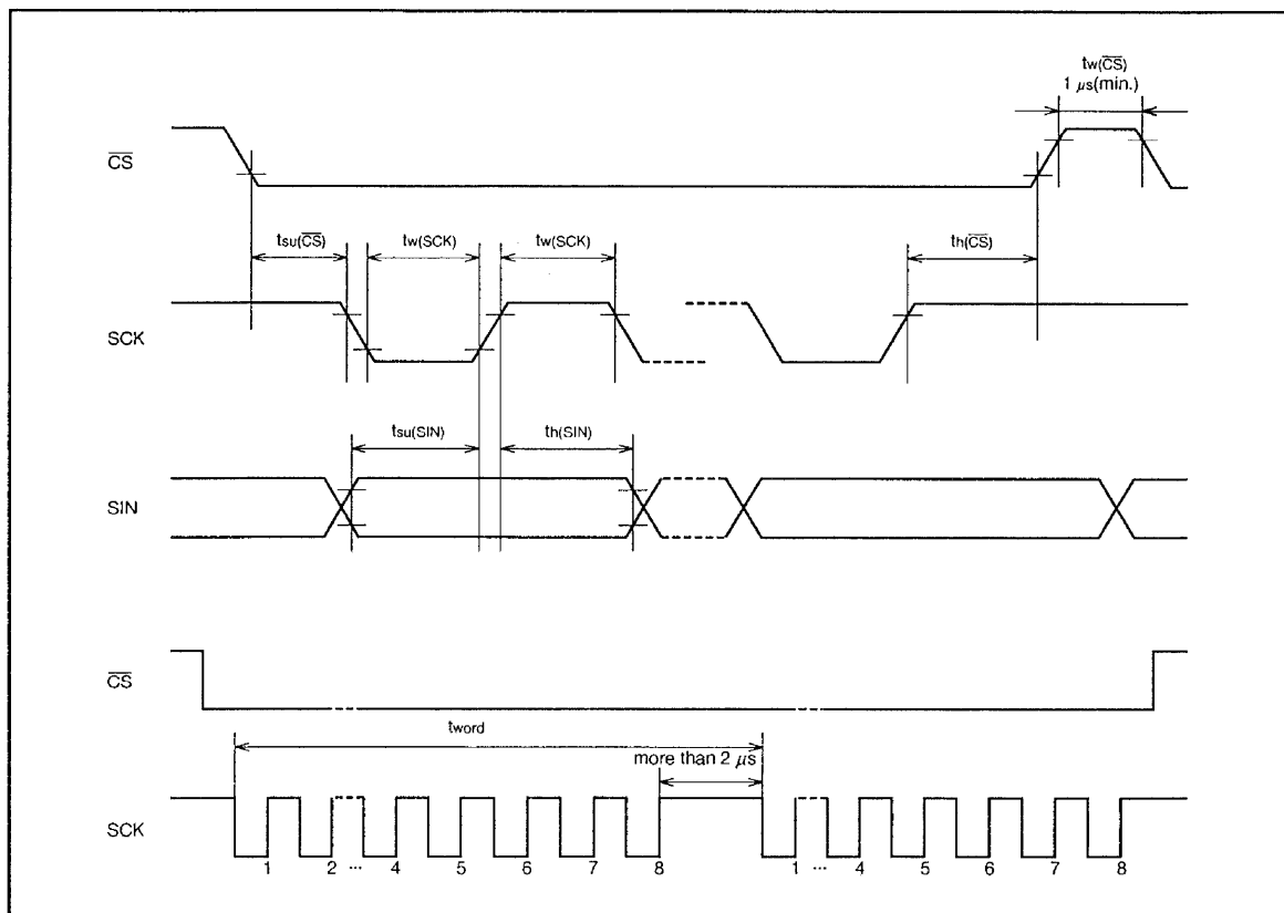
Fig. 10 Serial input timing requirements
