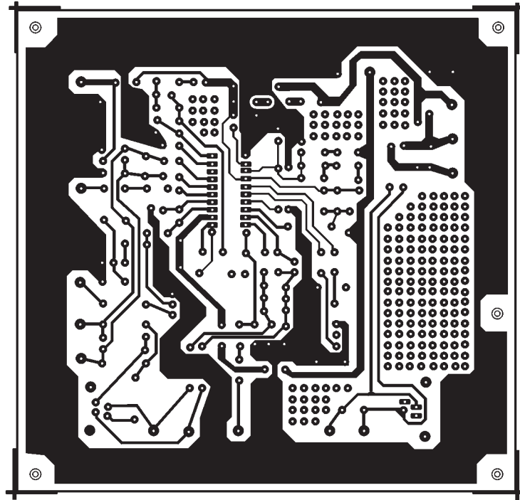
Soldering surface
