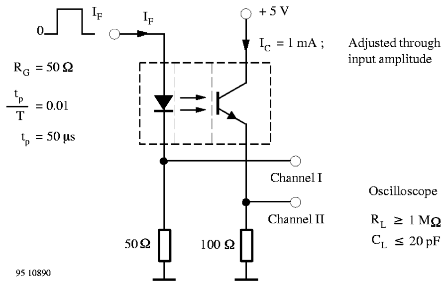
Figure 1. Test circuit
