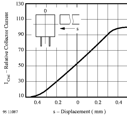
Figure 10. Relative Collector Current vs. Displacement
