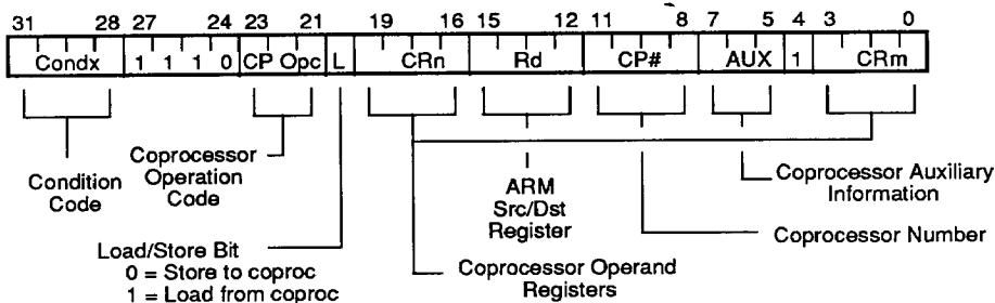
FIGURE 19. COPROCESSOR REGISTER TRANSFERS (MRC, MCR)
