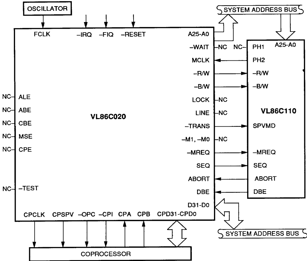
FIGURE 33. CONNECTING VL86C020 TO VL86C110 (MEMC)
