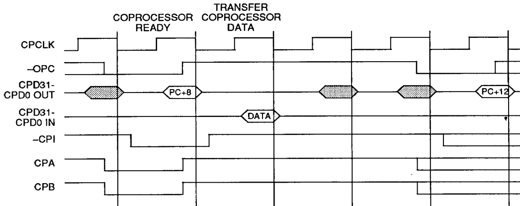
FIGURE 30. COPROCESSOR REGISTER TRANSFER (LOAD FROM COPROCESSOR)
