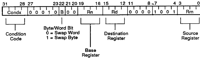
FIGURE 15. SINGLE DATA SWAP (SWP)
