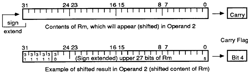
FIGURE 7. ARITHMETIC SHIFT RIGHT (ASR)
