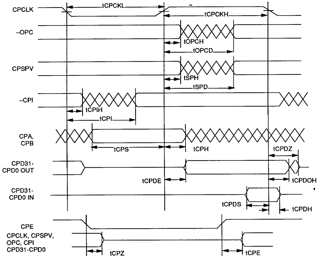
FIGURE 35. COPROCESSOR INTERFACE TIMING
