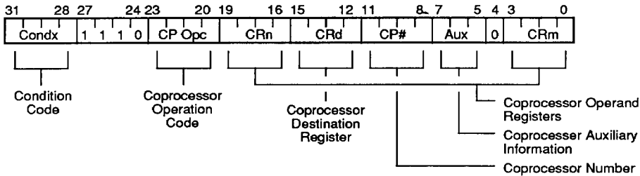
FIGURE 17. COPROCESSOR DATA OPERATIONS (CDO)
