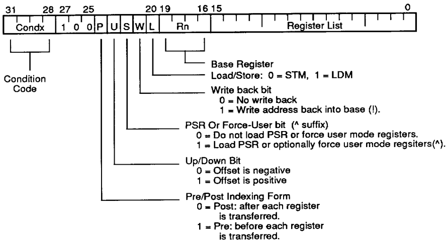
FIGURE 12. LOAD/STORE REGISTER LIST FROM MEMORY (LDM,STM)
