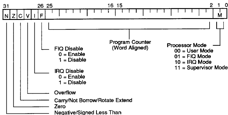
FIGURE 1. PROGRAM COUNTER AND PROCESSOR STATUS REGISTER
