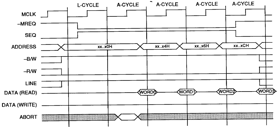
FIGURE 26. LINE FETCH OPERATION
