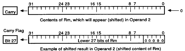
FIGURE 5. LOGICAL SHIFT LEFT (LSL)
