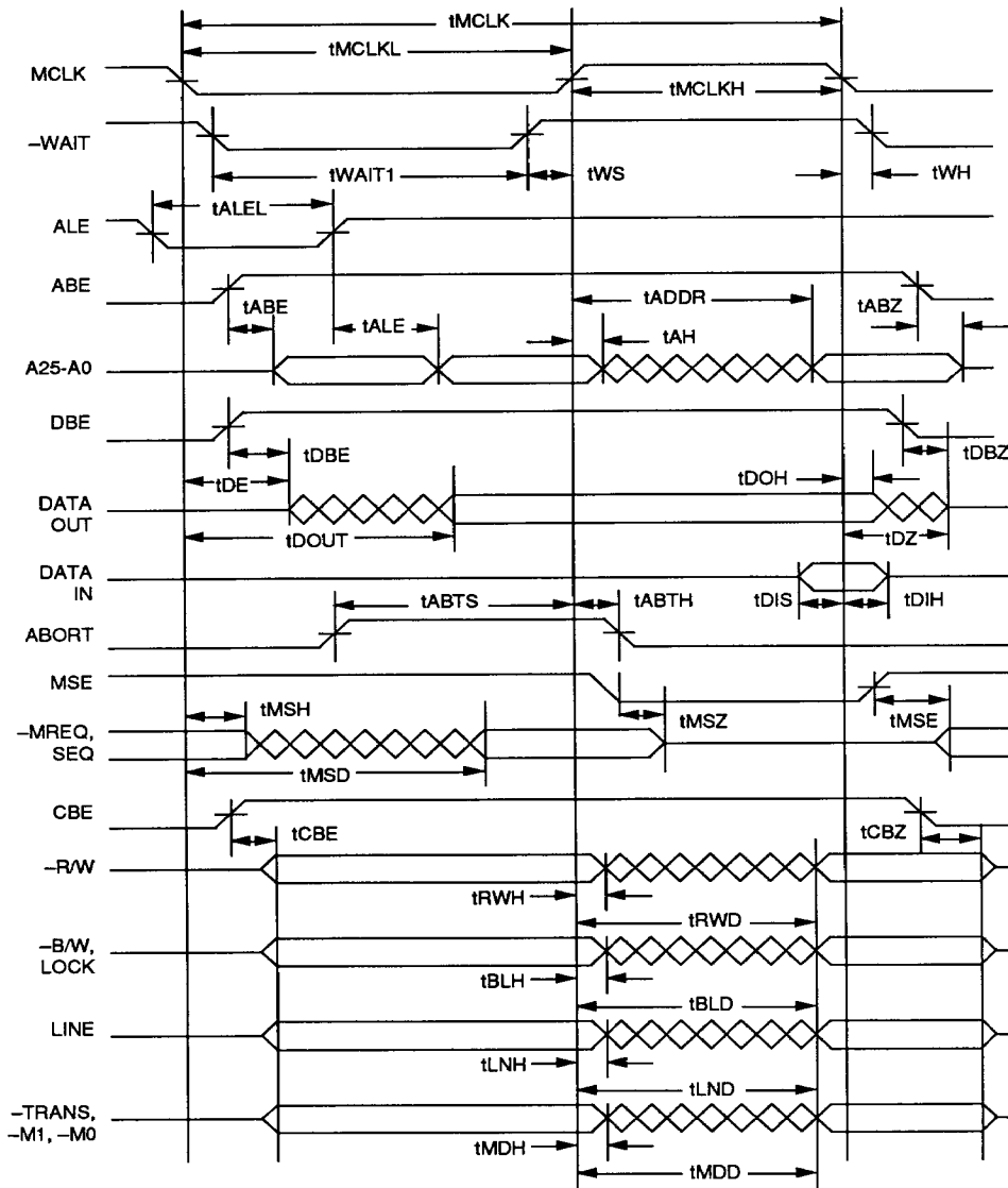
FIGURE 34. MEMORY INTERFACE TIMING
