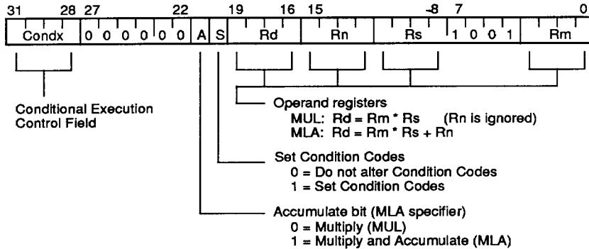
FIGURE 10. MULTIPLY AND MULTIPLY-ACCUMULATE (MUL, MLA)
