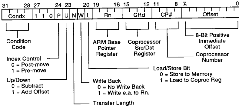
FIGURE 18. COPROCESSOR DATA TRANSFERS (LDC, STC)
