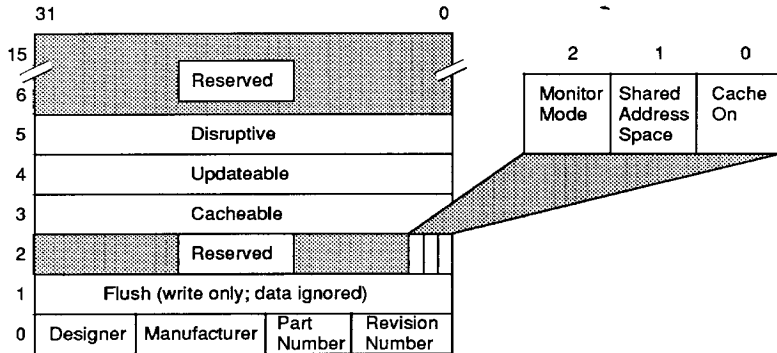
FIGURE 22. VL86C020 CONTROL REGISTERS
