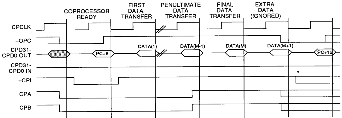
FIGURE 28. COPROCESSOR DATA TRANSFER (FROM MEMORY TO COPROCESSOR)
