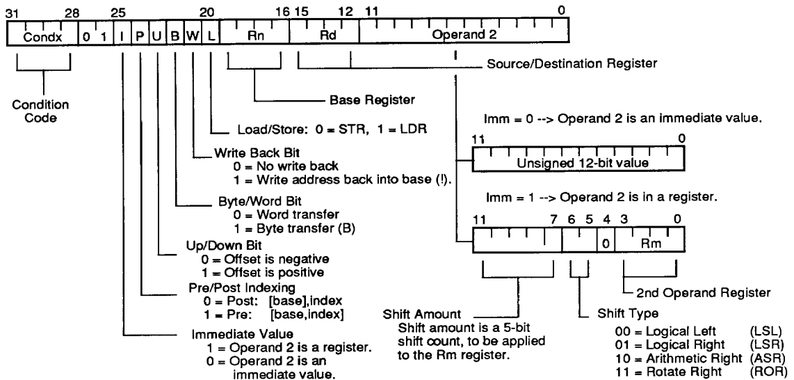
FIGURE 11. SINGLE DATA TRANSFER (LDR, STR)
