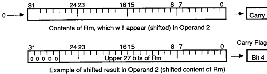
FIGURE 6. LOGICAL SHIFT RIGHT (LSR)
