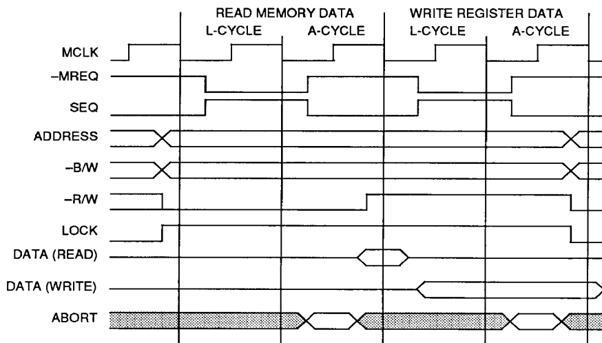
FIGURE 25. DATA SWAP OPERATION
