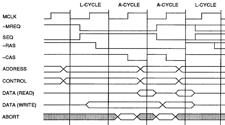
FIGURE 23. VL86C020 MEMORY TIMING
