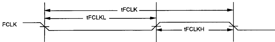
FIGURE 36. FCLK INTERFACE TIMING
