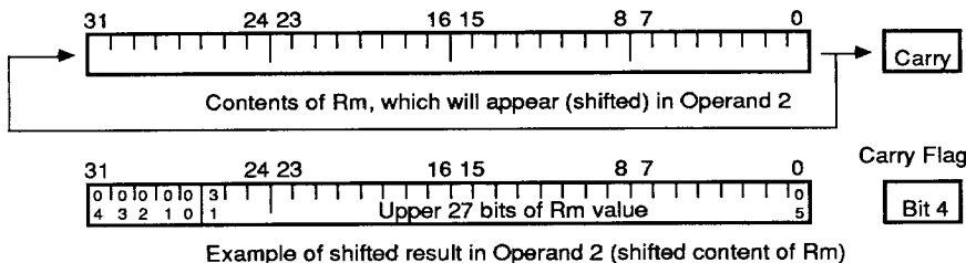
FIGURE 8. ROTATE RIGHT (ROR)
