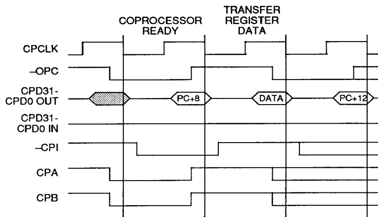
FIGURE 31. COPROCESSOR REGISTER TRANSFER (STORE TO COPROCESSOR)
