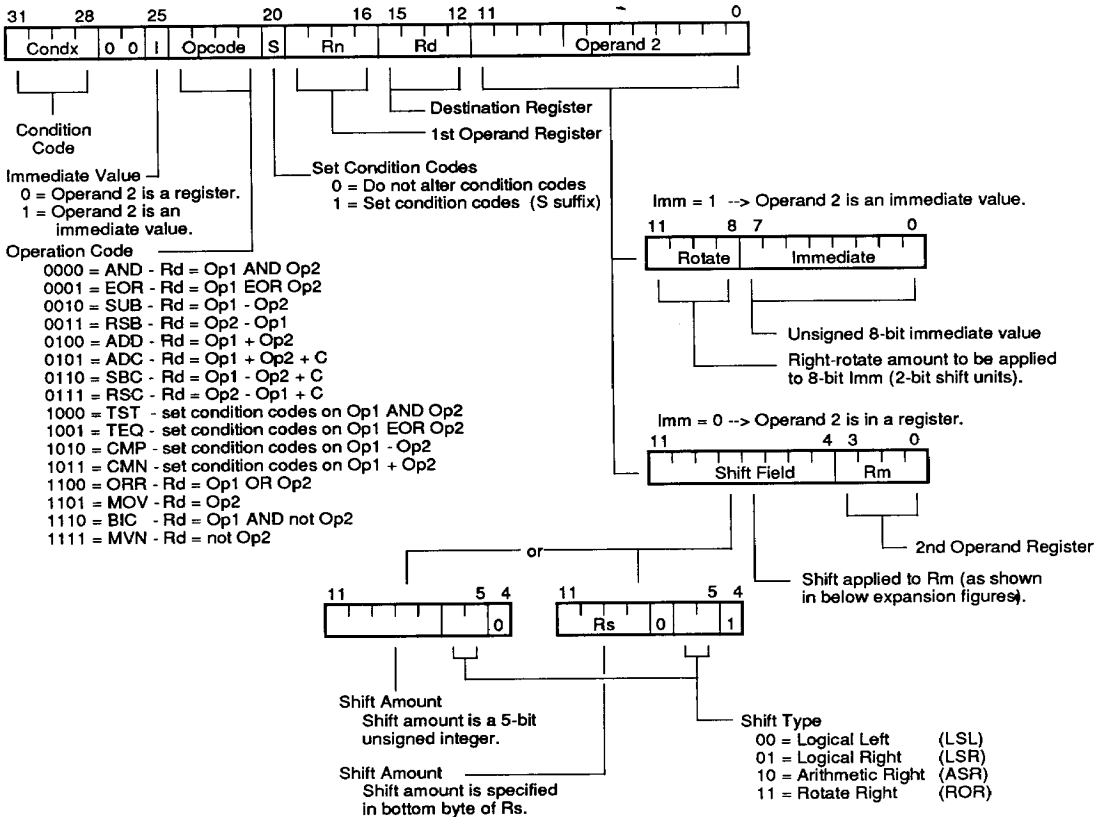
FIGURE 4. ALU INSTRUCTION TYPES
