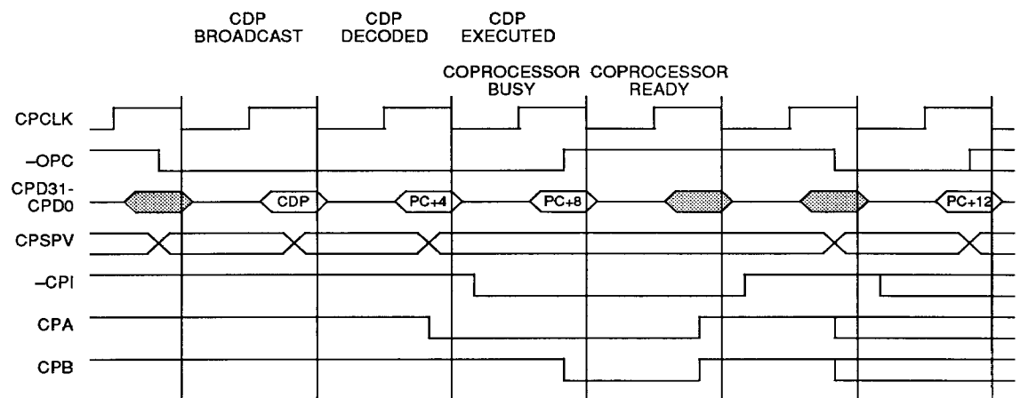
FIGURE 27. COPROCESSOR DATA OPERATION
