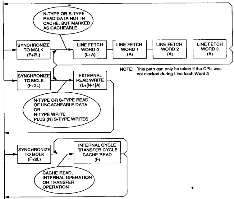
FIGURE 33. WORST-CASE VL86C020 TIMING FLOWCHART
