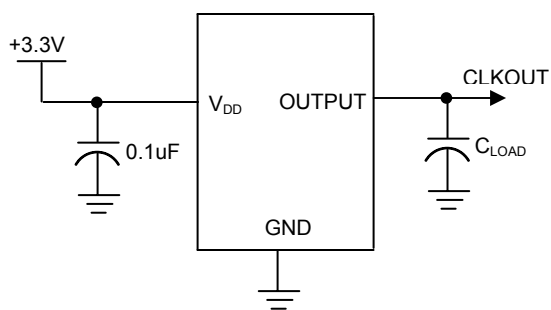
TEST CIRCUIT #1
