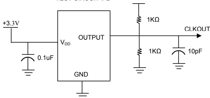
TEST CIRCUIT # 2
