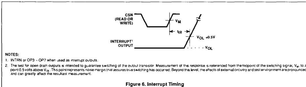
Figure 6. Interrupt Timing
