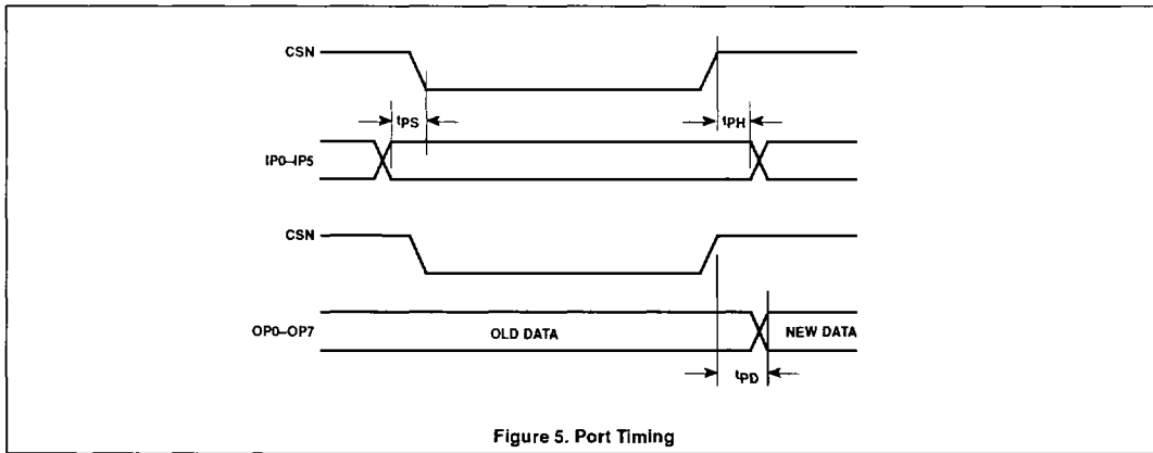
Figure 5. Port Timing
