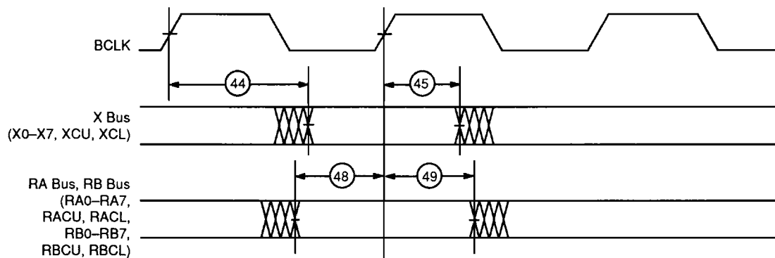
Figure 40. PHY Interface Timings
