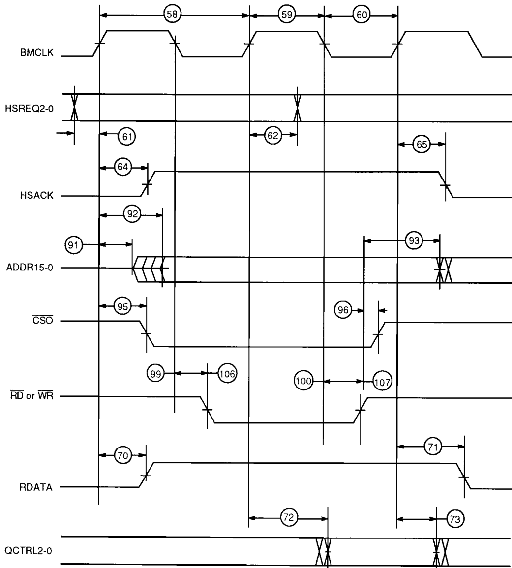
Figure 41. Host Interface Signal Timings
