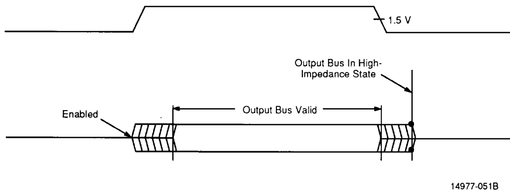
Figure 47. Output Waveform Test Points
