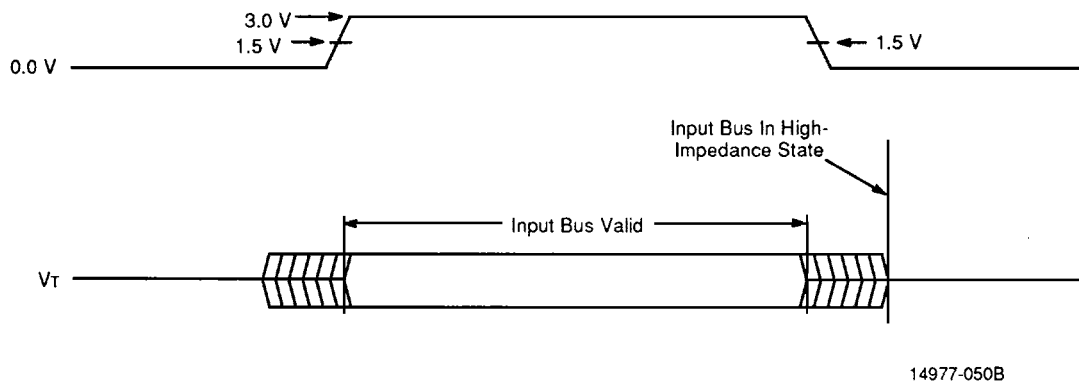
Figure 46. Input Waveform Test Points
