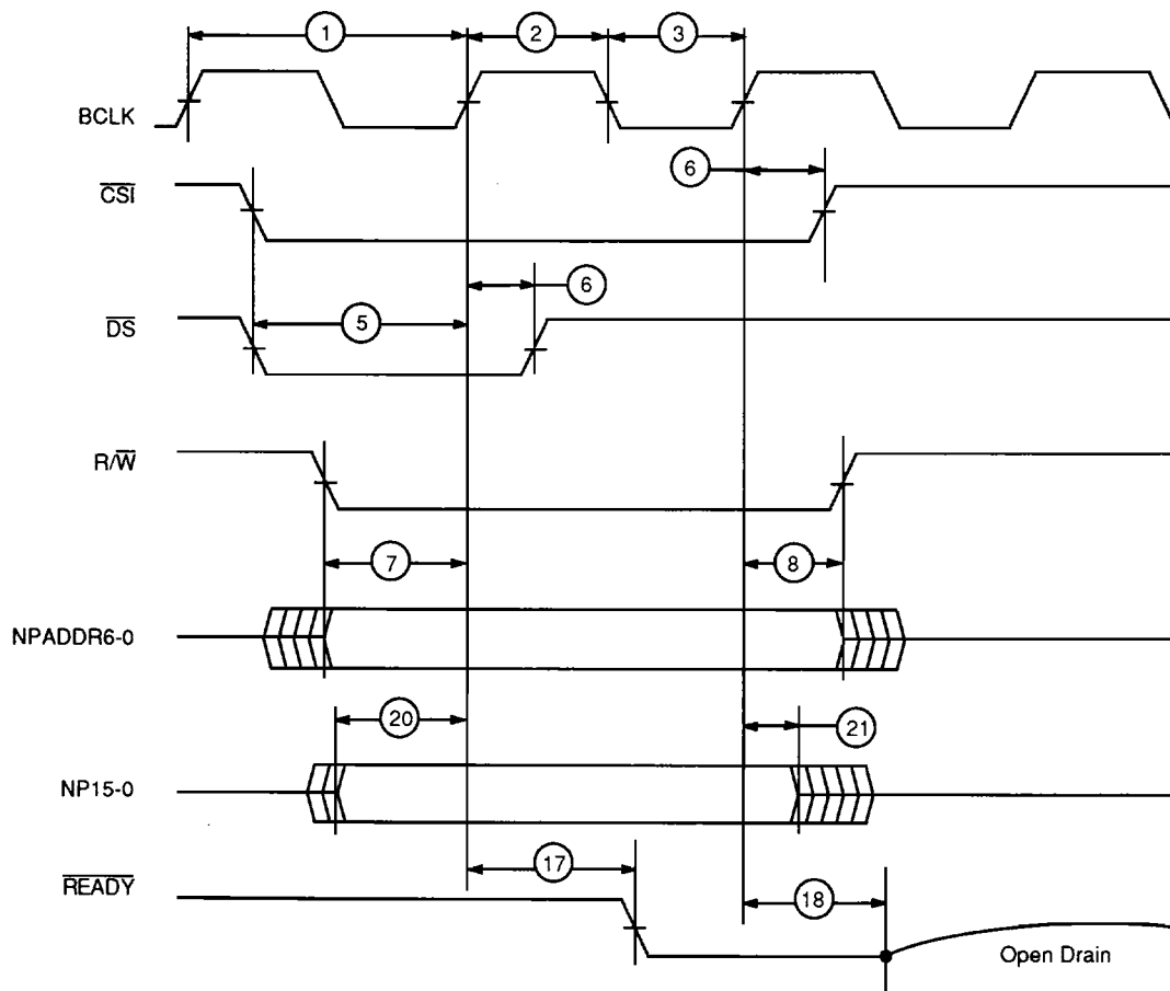
Figure 37. NP Bus Synchronous Write Timings
