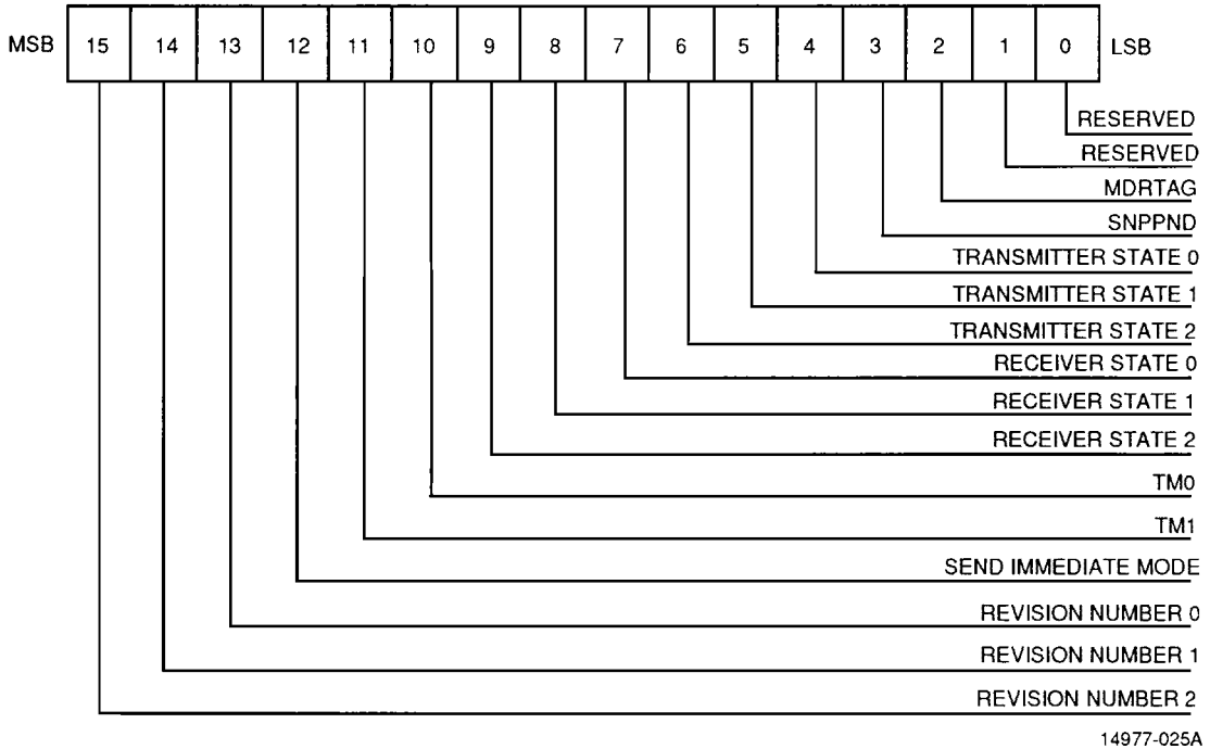
Figure 22. State Machine Register
