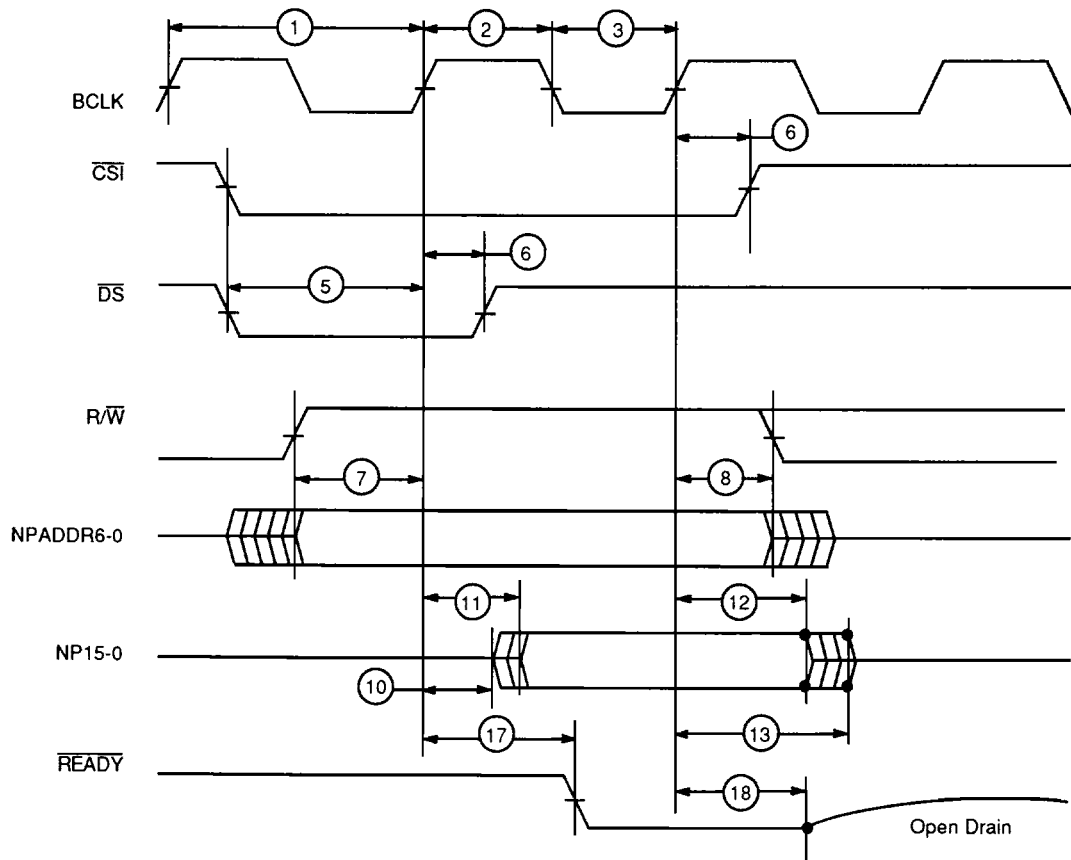
Figure 36. NP-Bus Synchronous Read Timings
