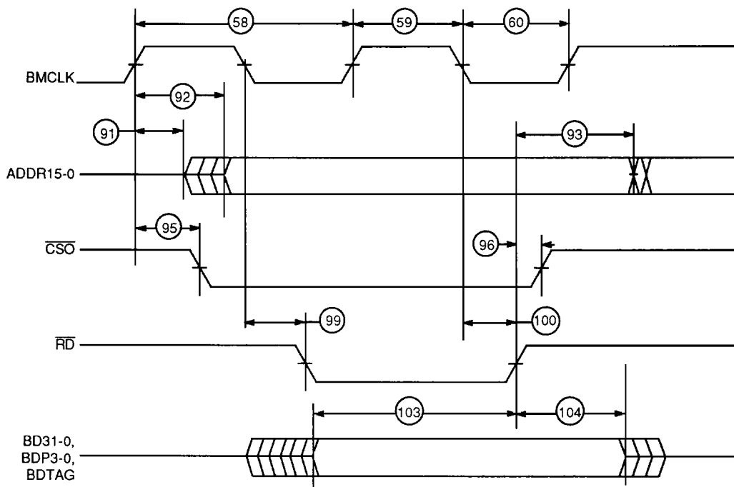
Figure 42. Buffer Memory Read Cycle Timings
