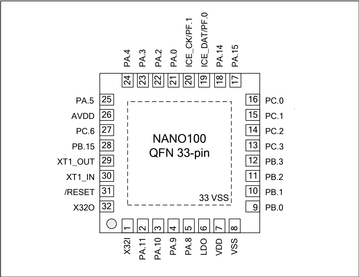
Figure 3-5 NuMicro™ Nano100 QFN 33-pin Assignment
