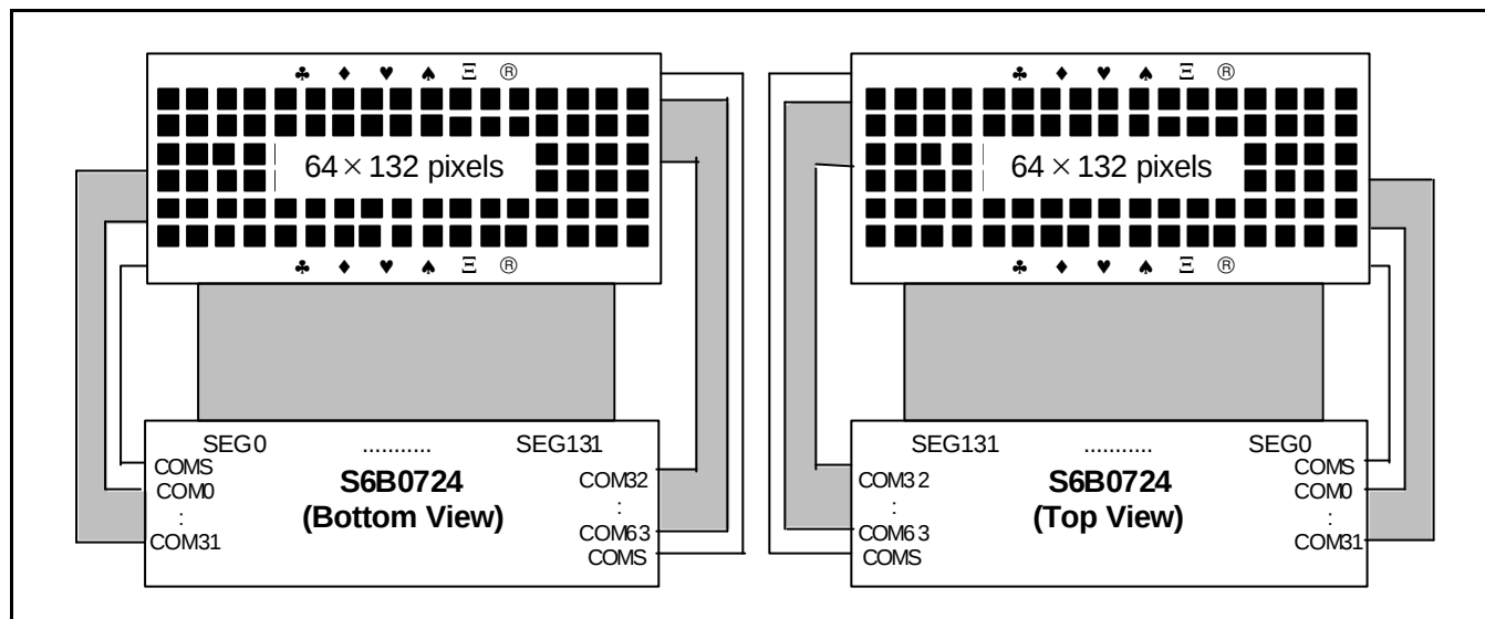
Figure 40. SHL = 1, ADC = 0
