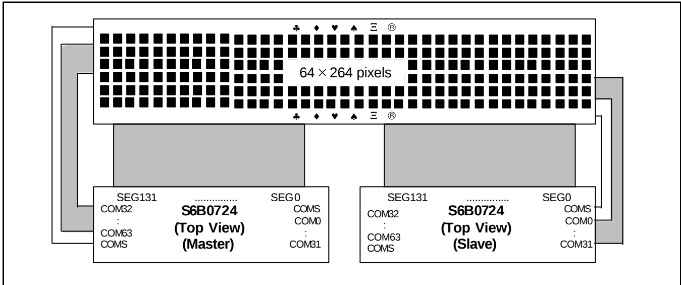
Figure 56. SHL = 1, ADC = 1
