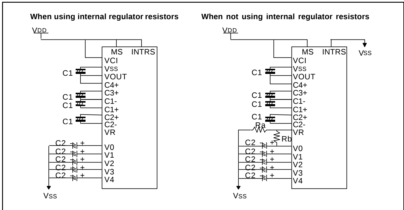
Figure 19. When Using all Internal LCD Power Circuits (VCI = VDD, 4-time V/I: ON, V/R: ON, V/F: ON)
