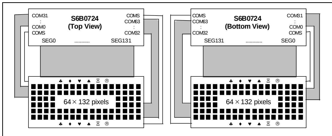
Figure 42. SHL = 0, ADC = 0
