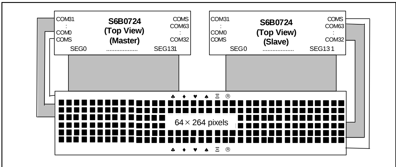
Figure 57. SHL = 0, ADC = 0
