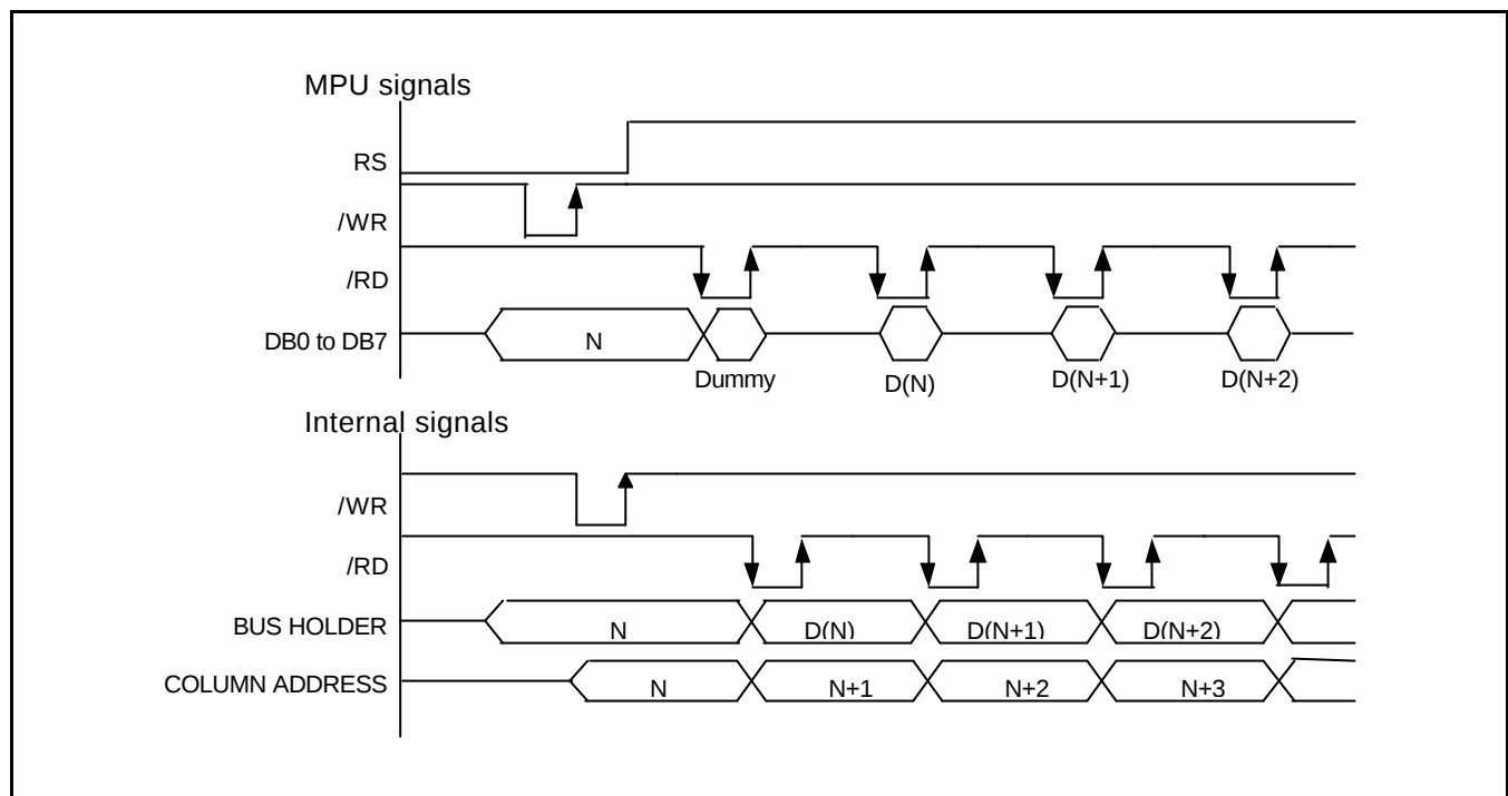
Figure 7. Read Timing
