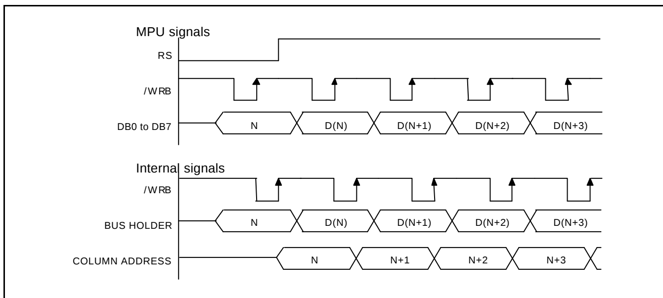
Figure 6. Write Timing
