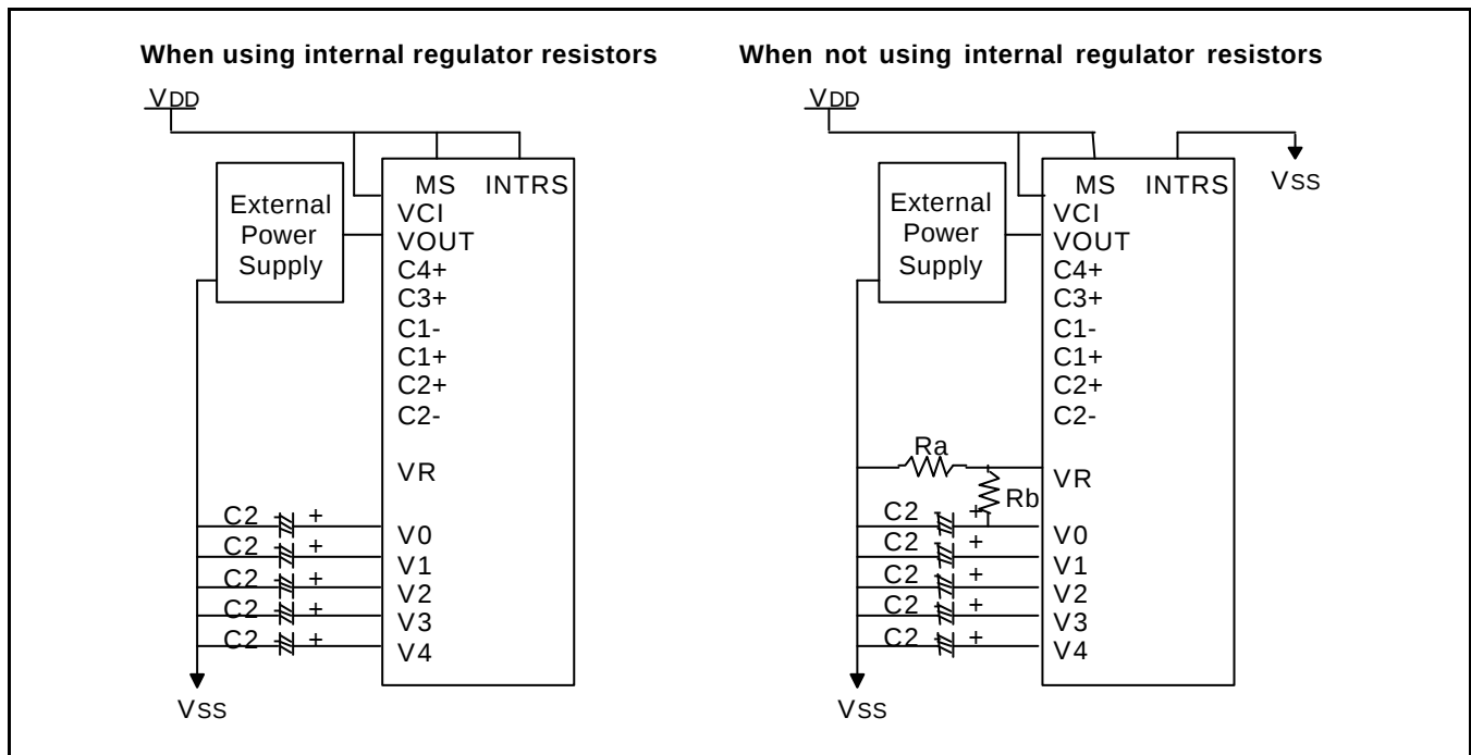
Figure 20. When Using some Internal LCD Power Circuits (VCI = VDD, V/I: OFF, V/R: ON, V/F: ON)
