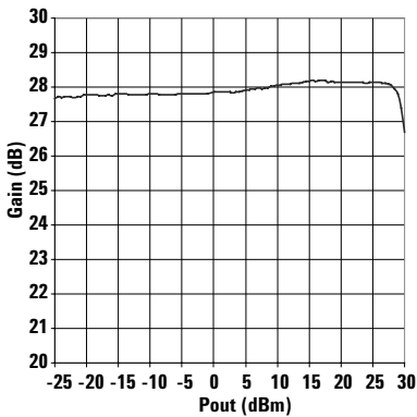
Figure 10. Gain vs Pout
