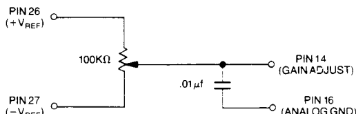
FIGURE 4. OFFSET TRIM
