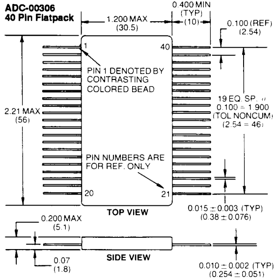
FIGURE 6. MECHANICAL OUTLINES
