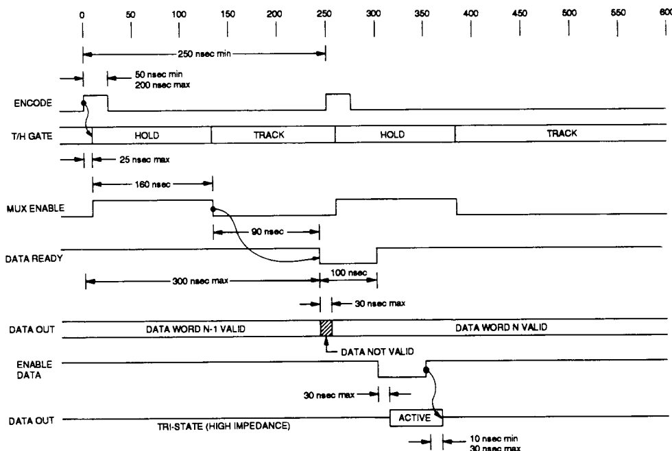
FIGURE 2. ADC-00304 TIMING DIAGRAM
