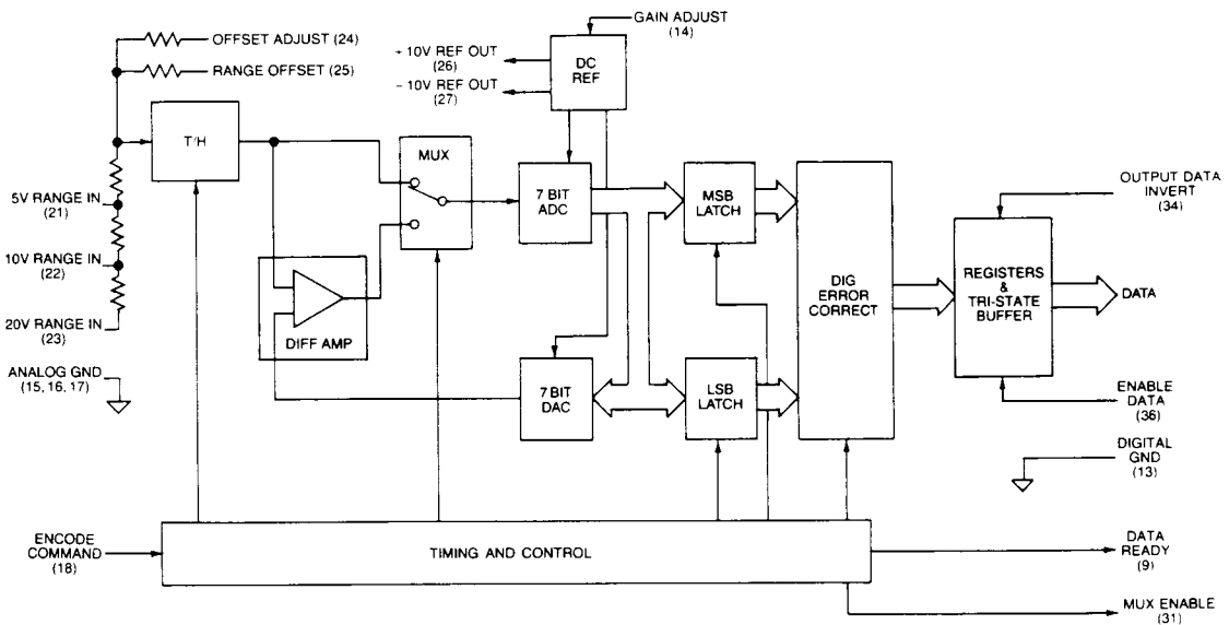
FIGURE 1. ADC-00304 BLOCK DIAGRAM
