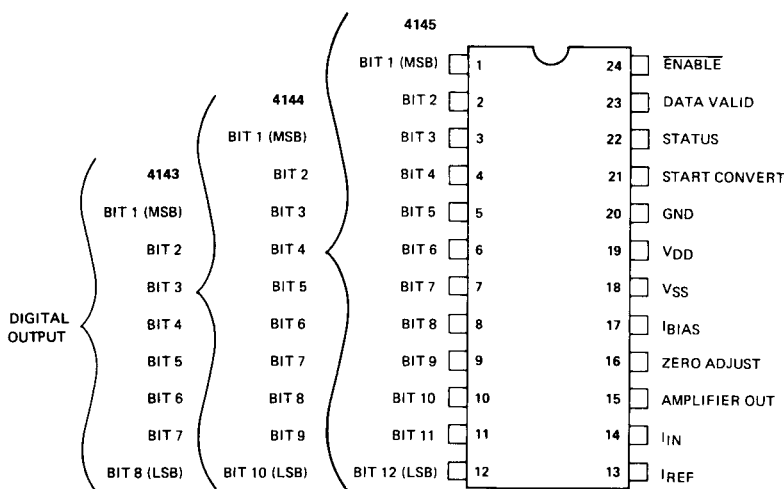
Figure 1. Pin Designations
