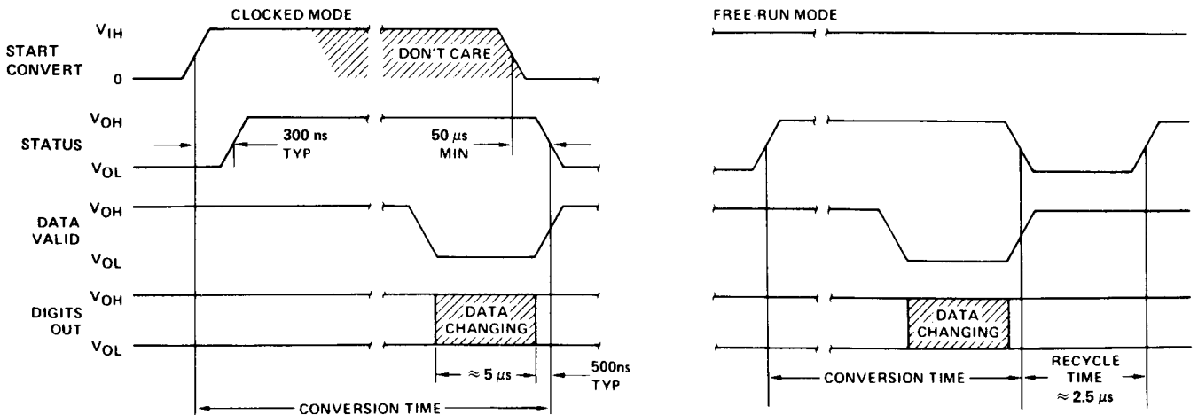
Figure 4. Timing Diagram (Rise, fall times = 200 ns typ., C_L = 50 pF)
