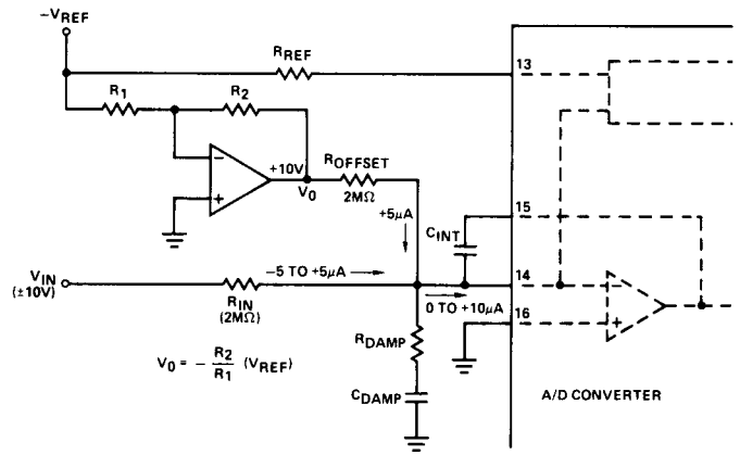
Figure 3. Offset Binary
